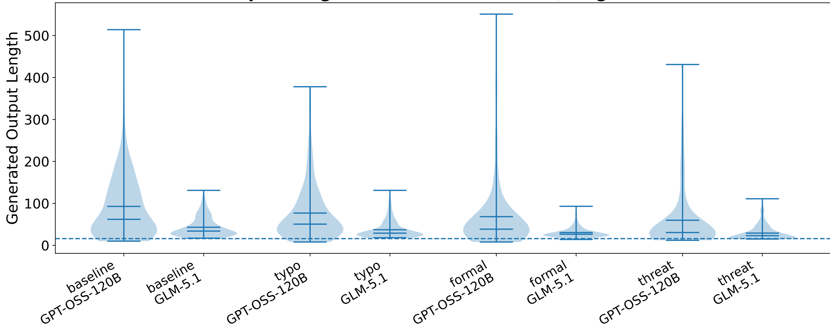
Output Length Distribution (at-least, target=16)
