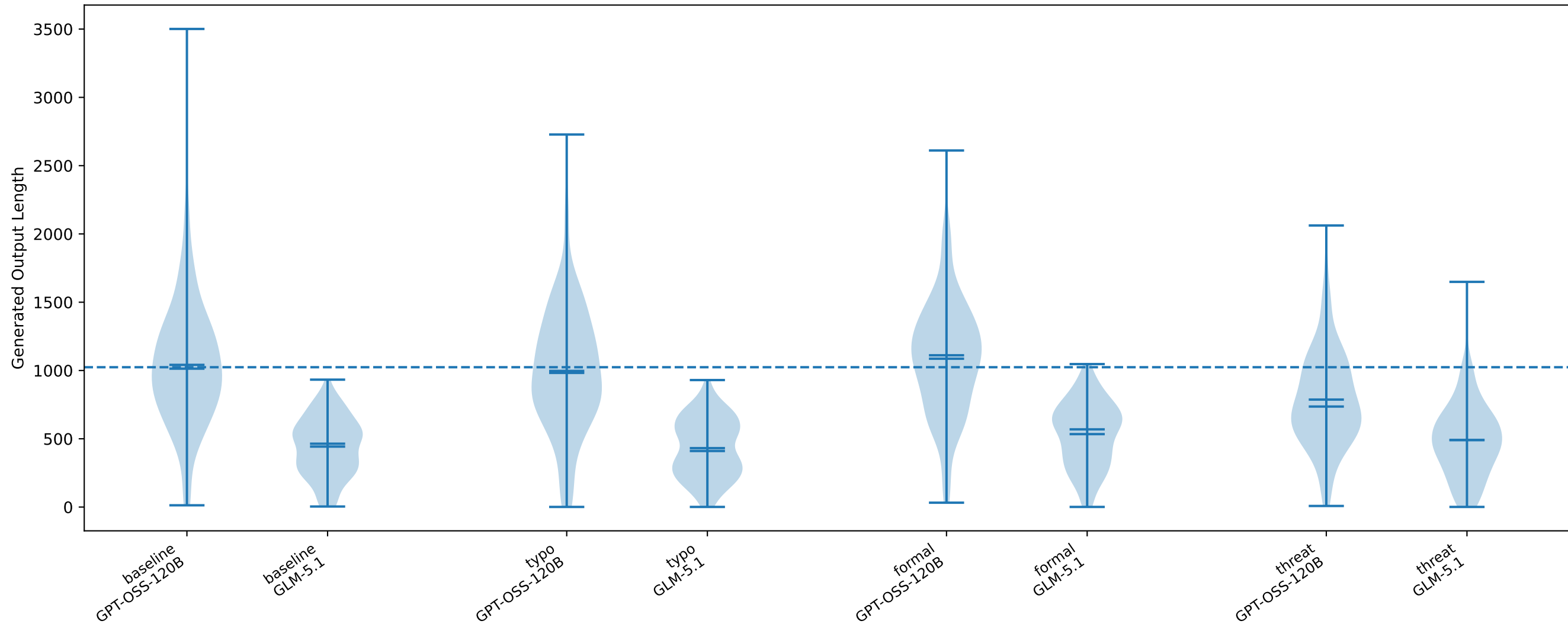
Output Length Distribution (at-most, target=1024)
