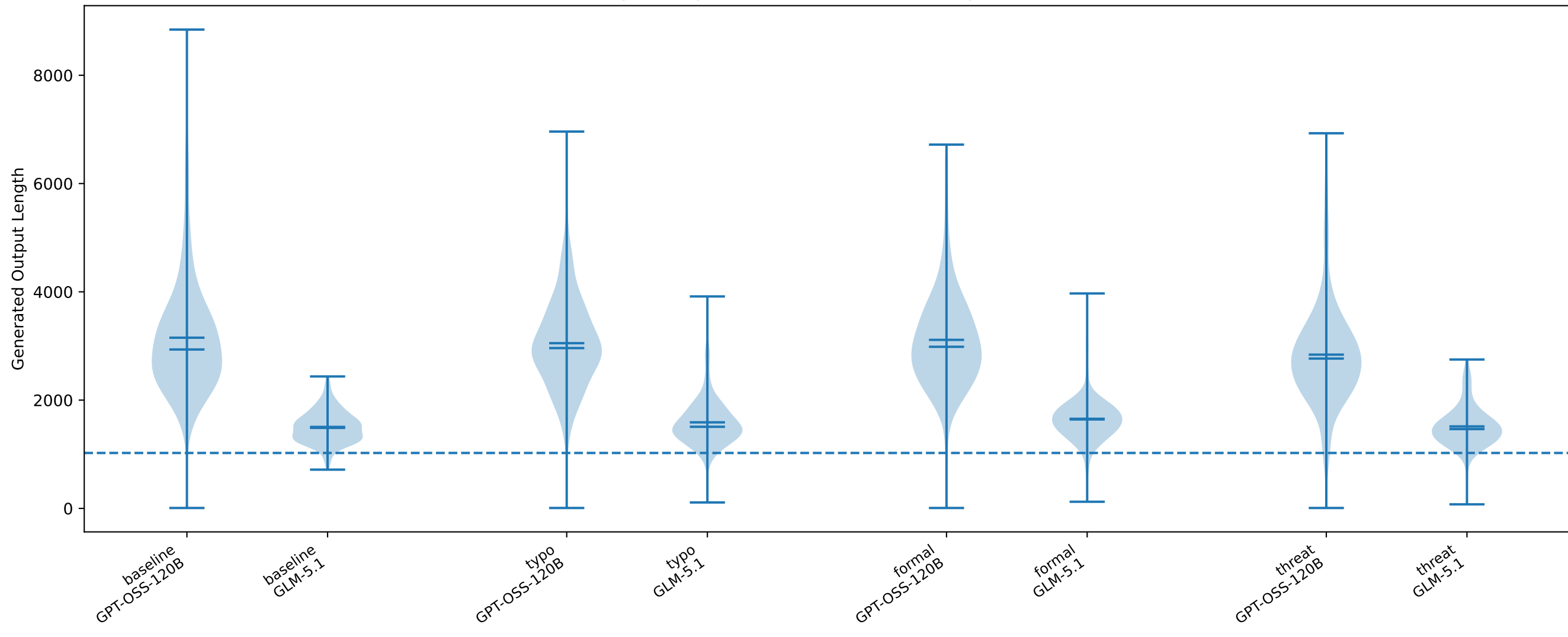
Output Length Distribution (at-least, target=1024)
