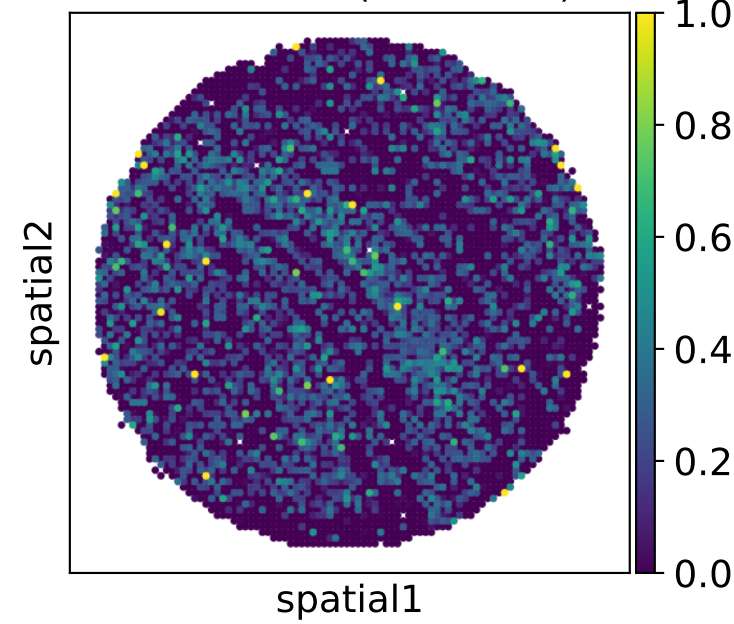
Iteration 10 (PCC=0.88)
