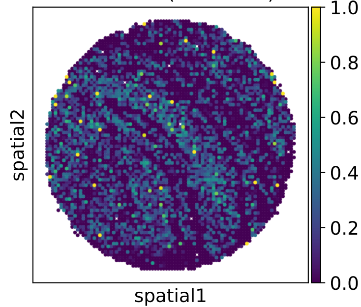
Iteration 1 (PCC=0.91)
