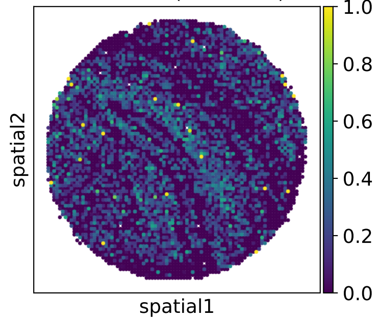
Iteration 4 (PCC=0.87)
