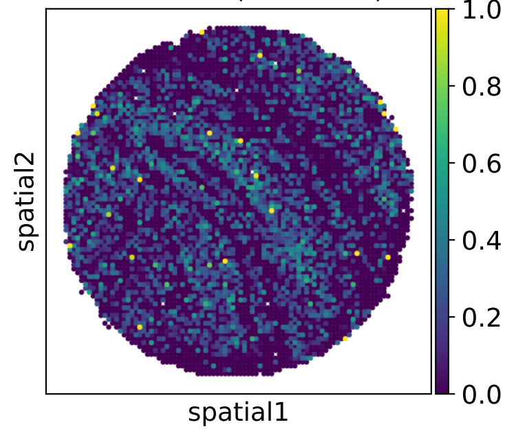
Iteration 5 (PCC=0.87)
