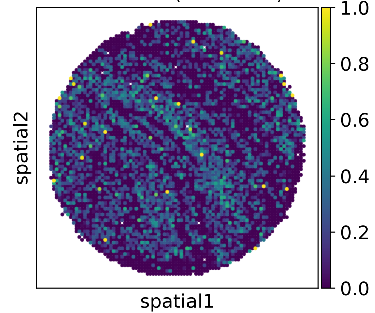
Iteration 3 (PCC=0.87)
