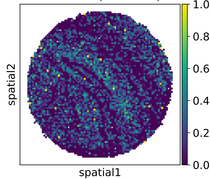
Iteration 2 (PCC=0.88)
