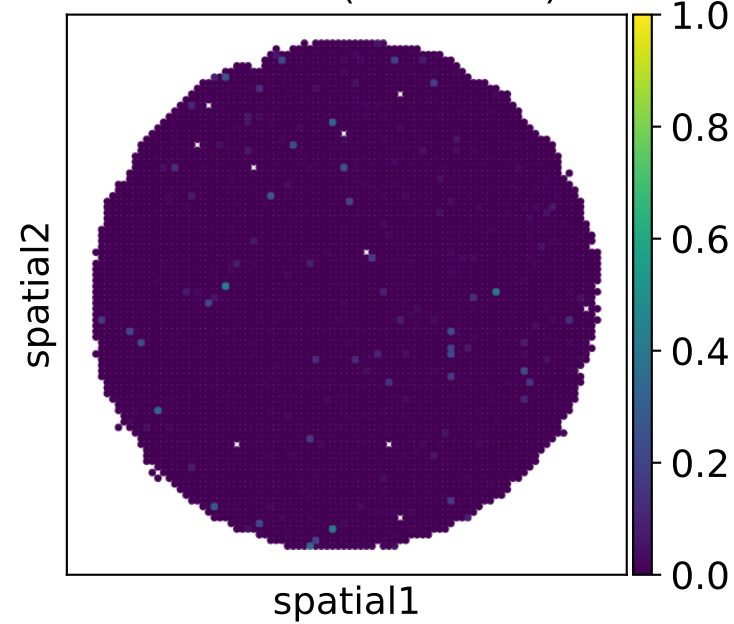
Iteration 2 (PCC=0.77)
