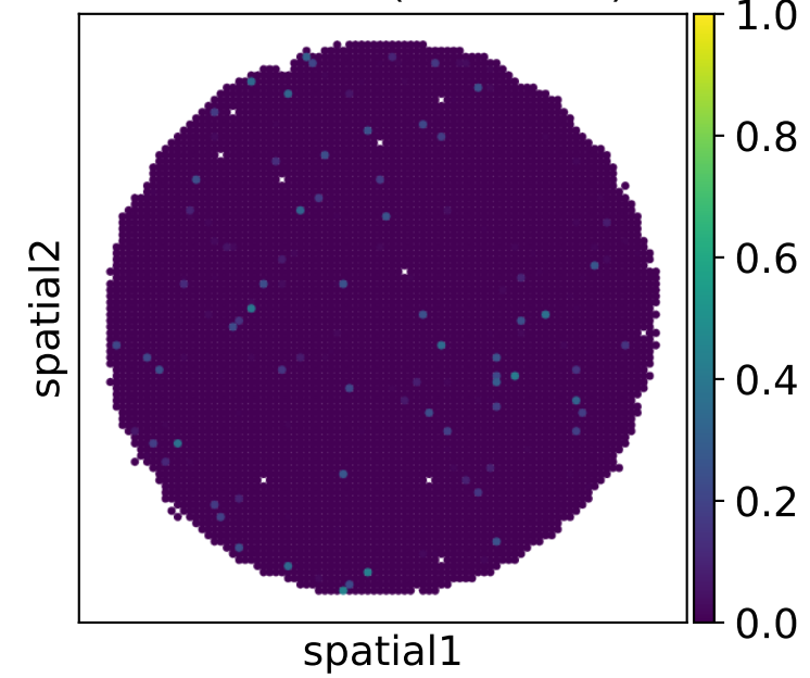
Iteration 20 (PCC=0.84)
