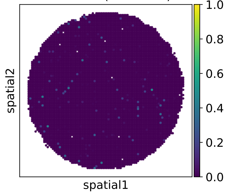
Iteration 1 (PCC=0.76)
