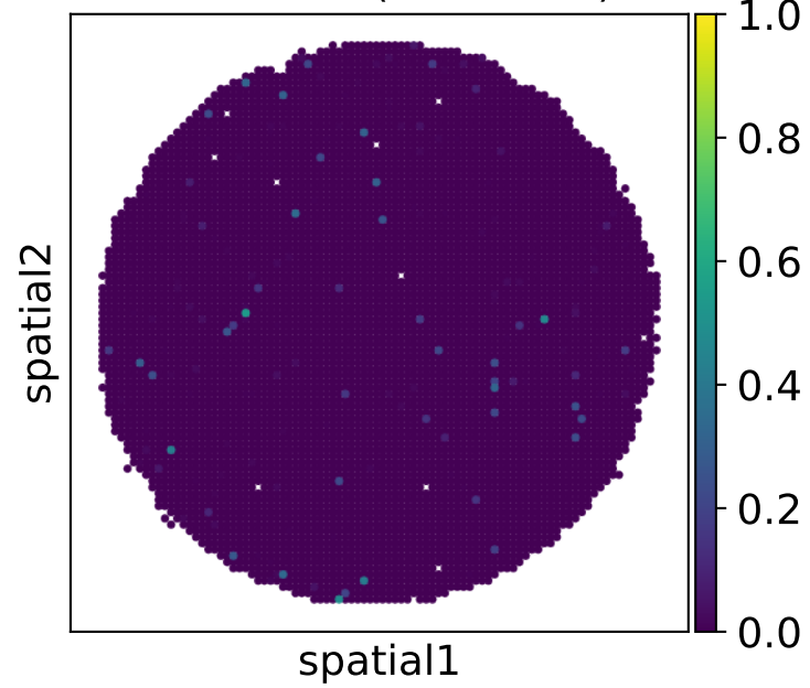
Iteration 5 (PCC=0.79)
