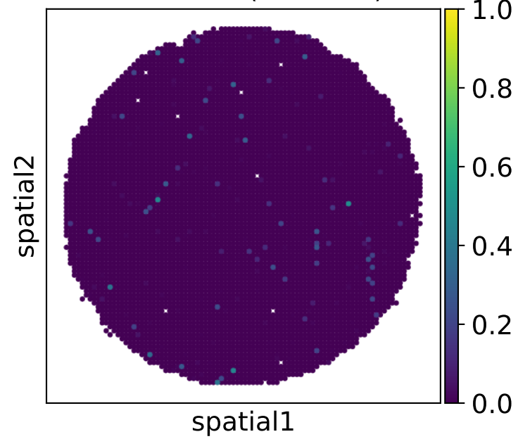
Iteration 4 (PCC=0.8)
