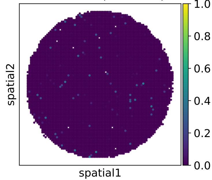
Iteration 10 (PCC=0.84)
