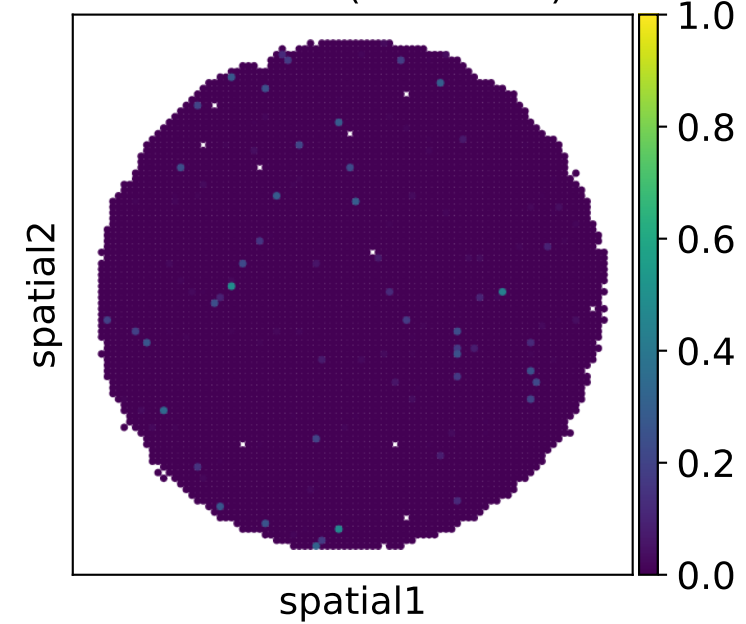
Iteration 3 (PCC=0.81)
