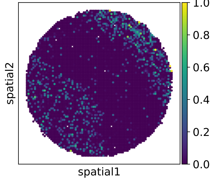
Iteration 5 (PCC=0.86)
