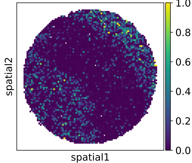
Iteration 1 (PCC=0.83)
