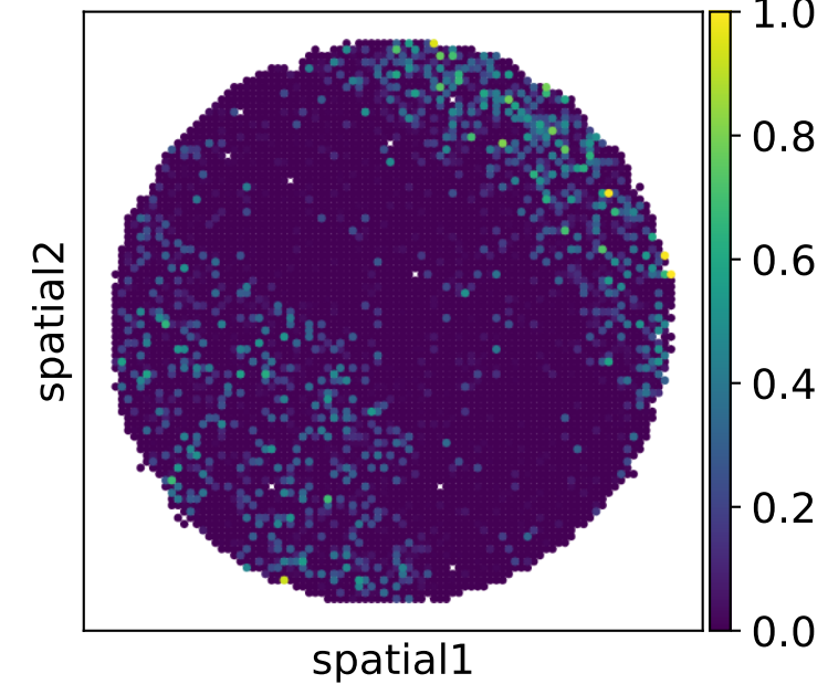
Iteration 3 (PCC=0.85)
