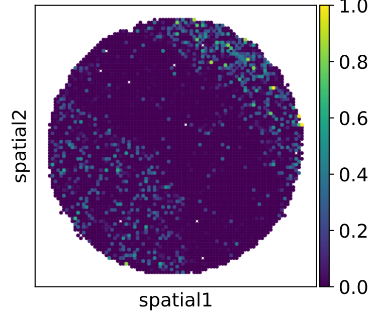
Iteration 2 (PCC=0.84)
