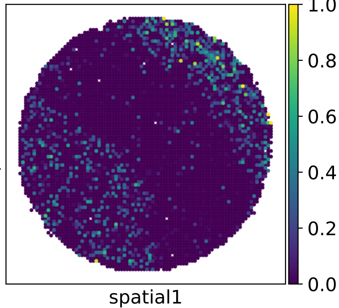
Iteration 4 (PCC=0.86)
