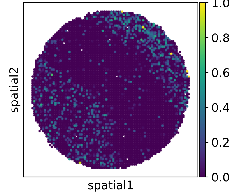
Iteration 20 (PCC=0.88)
