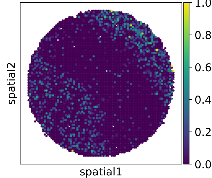
Iteration 10 (PCC=0.87)
