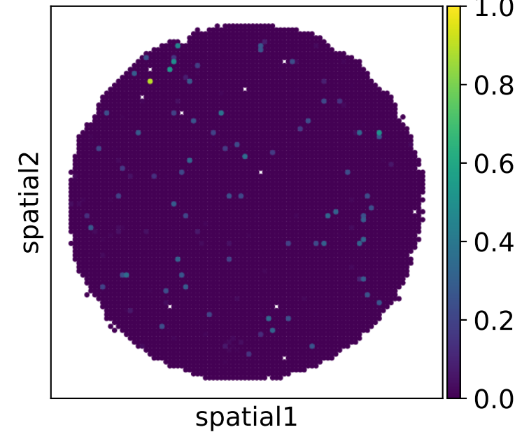
Iteration 20 (PCC=0.9)
