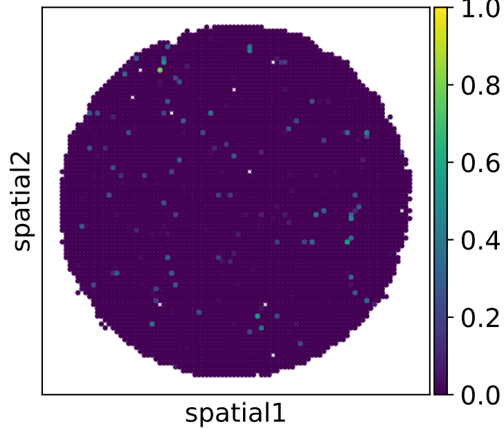
Iteration 1 (PCC=0.78)
