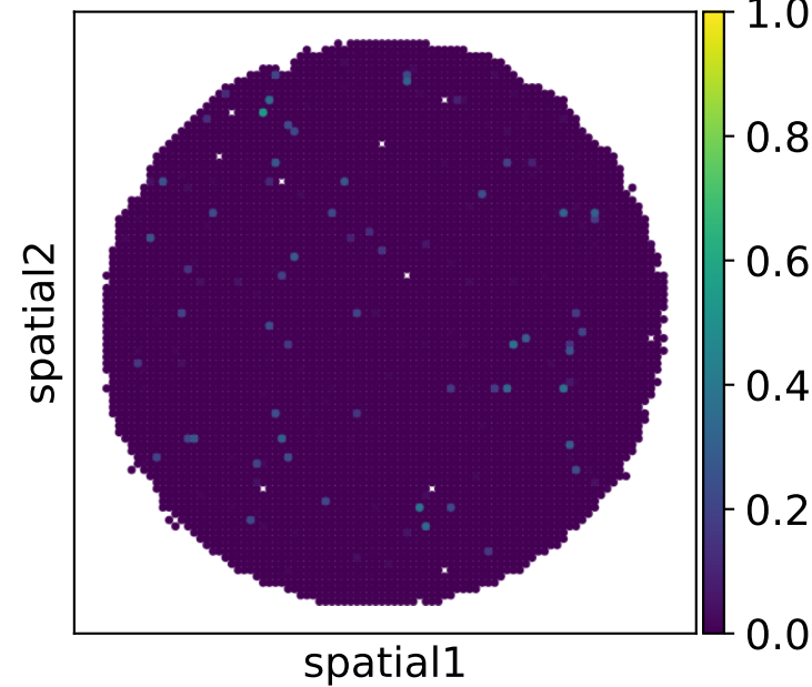
Iteration 2 (PCC=0.73)
