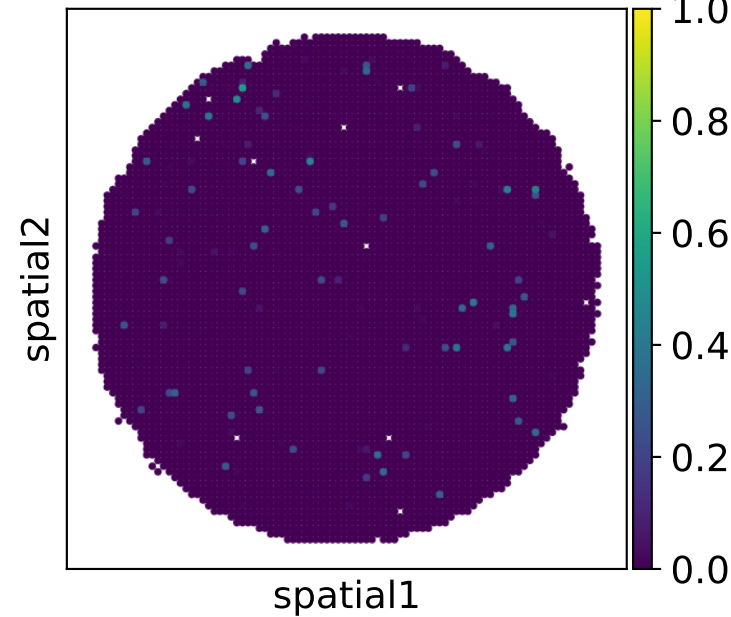
Iteration 10 (PCC=0.84)
