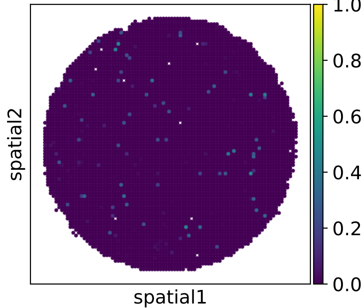
Iteration 5 (PCC=0.75)
