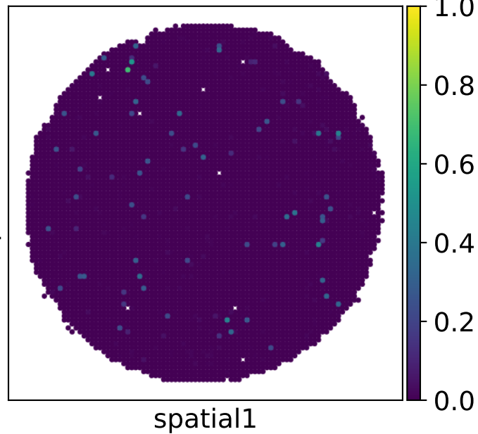
Iteration 4 (PCC=0.78)
