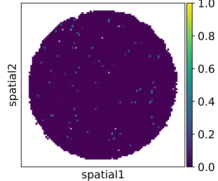
Iteration 3 (PCC=0.77)
