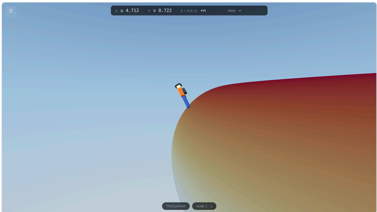
Figure 9. Standing on a torus. There is no height function here and no contours, but there is a normal at every point, and the explorer stands along it.
