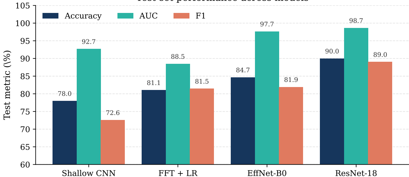
Test-set performance across models
