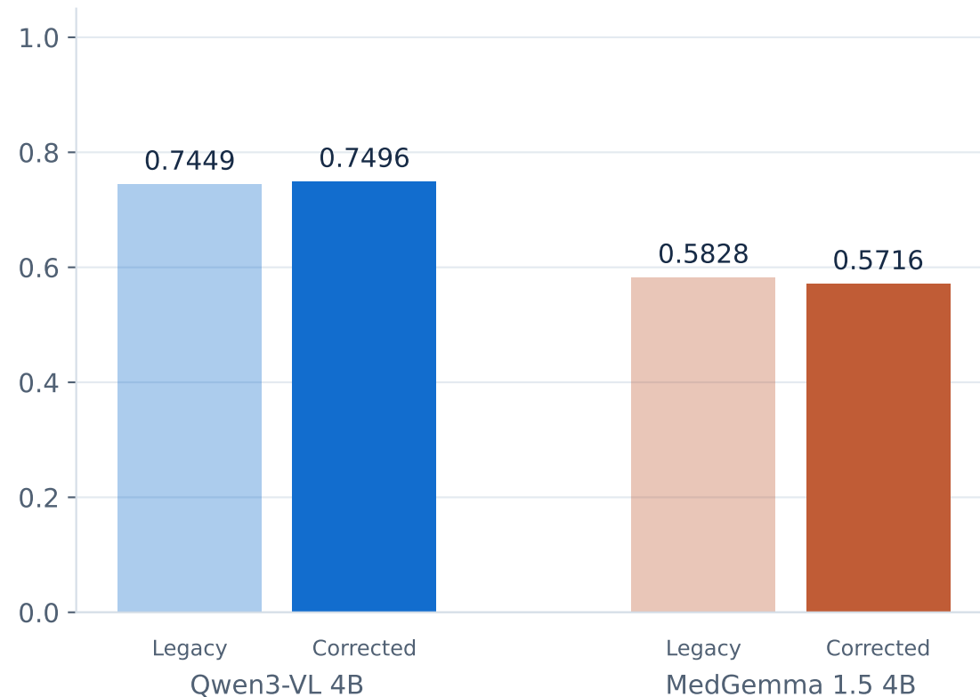
Mean intersection-over-union
