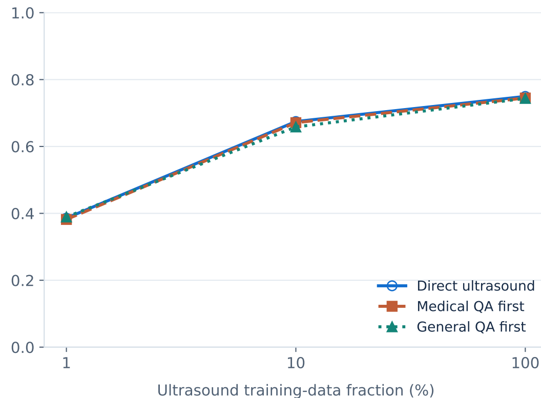
Mean grounding intersection-over-union
