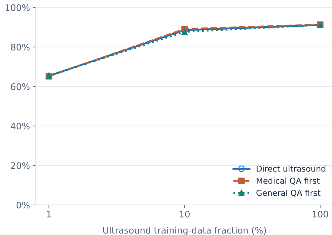
Converted open-QA exact match
