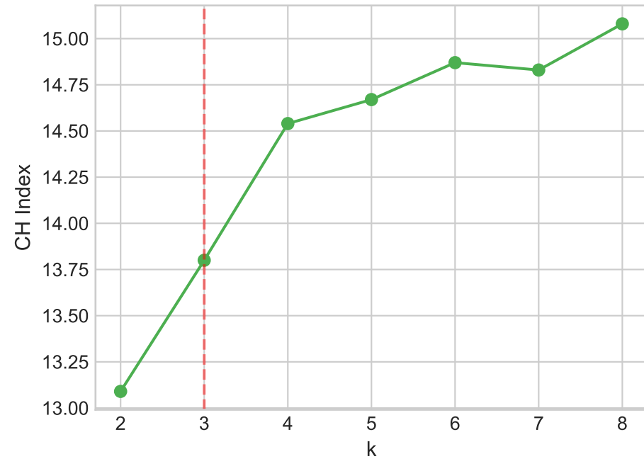
Calinski-Harabasz Index
