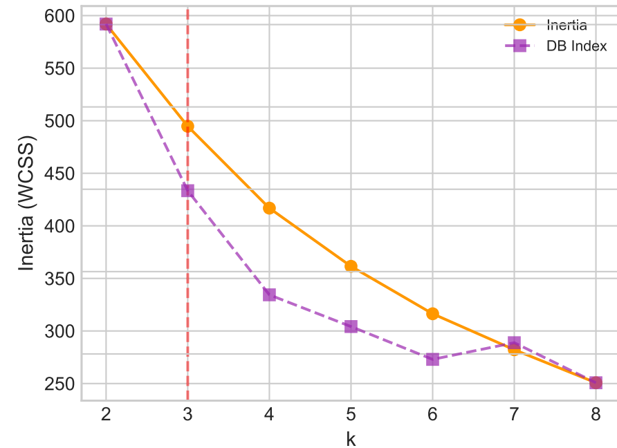
Elbow Method
