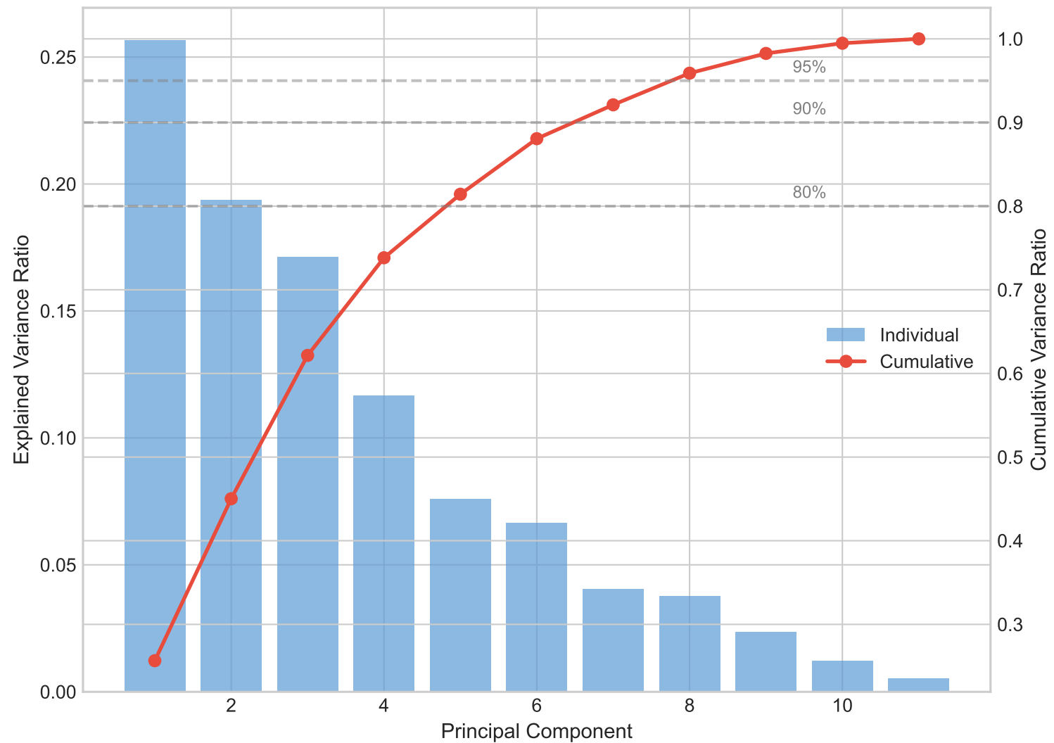
PCA Scree Plot
