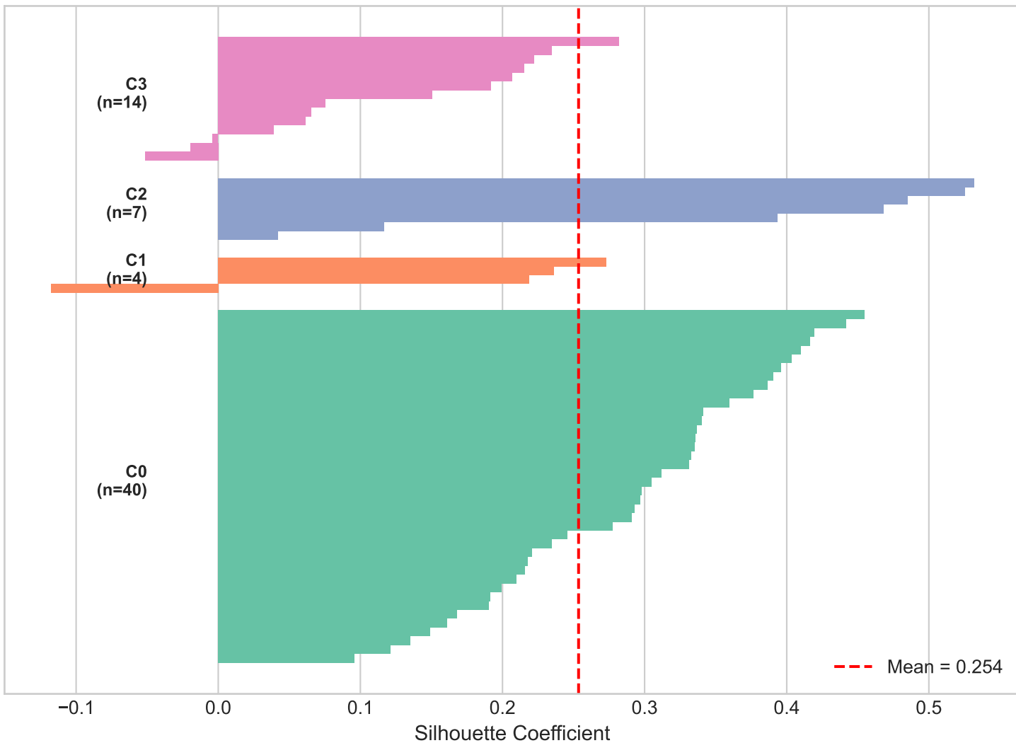
Silhouette Diagram (k=4)
