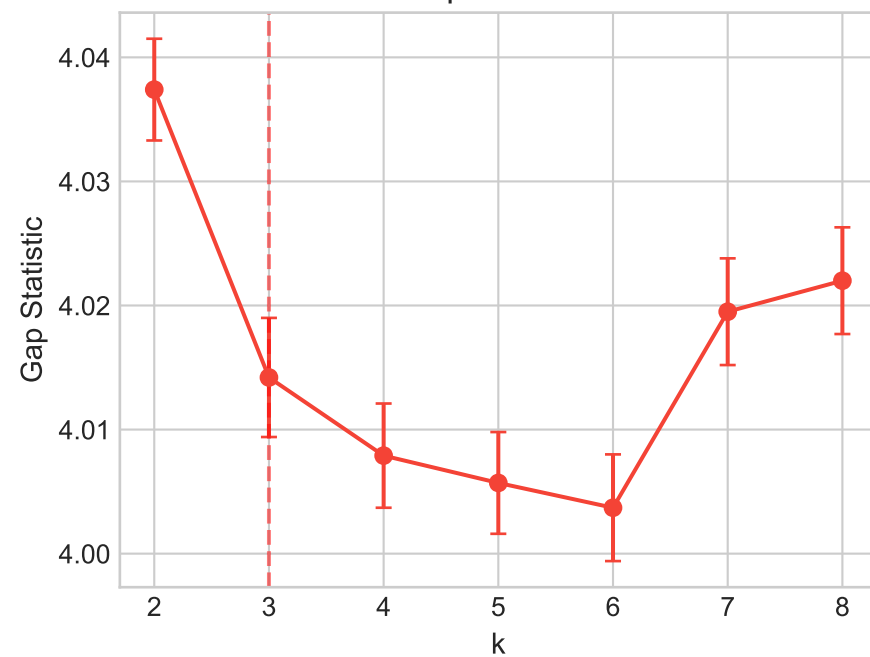
Gap Statistic
