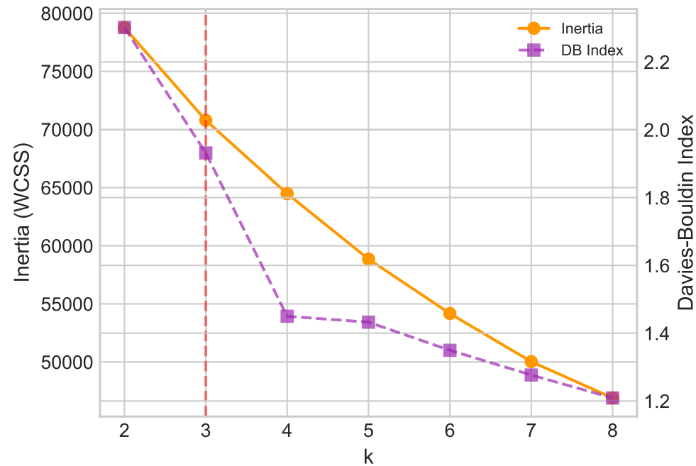
Elbow Method
