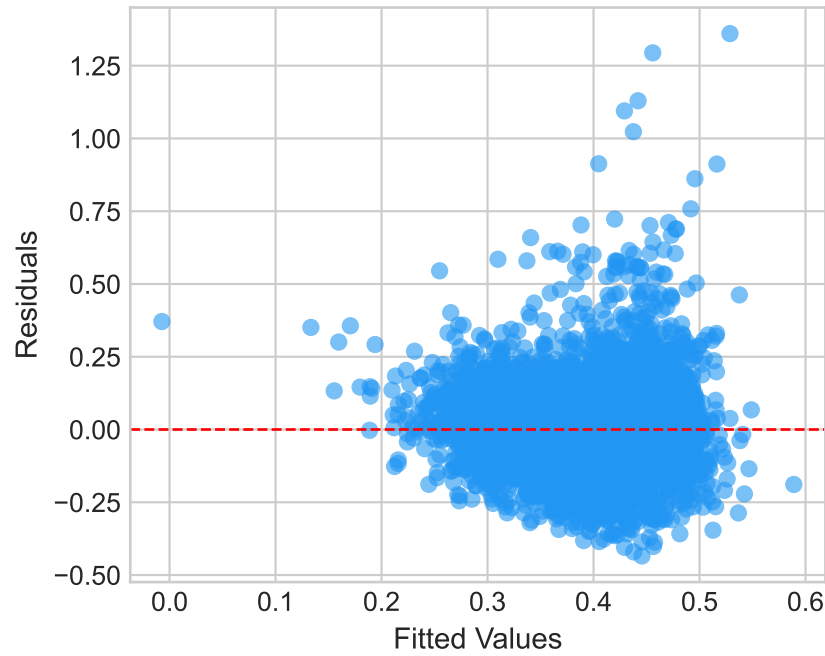
Residual Distribution
