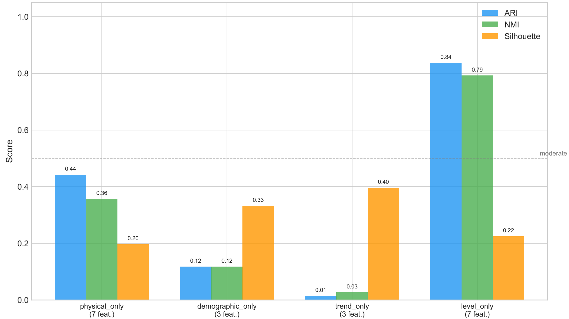
Specification Robustness (k=3)
