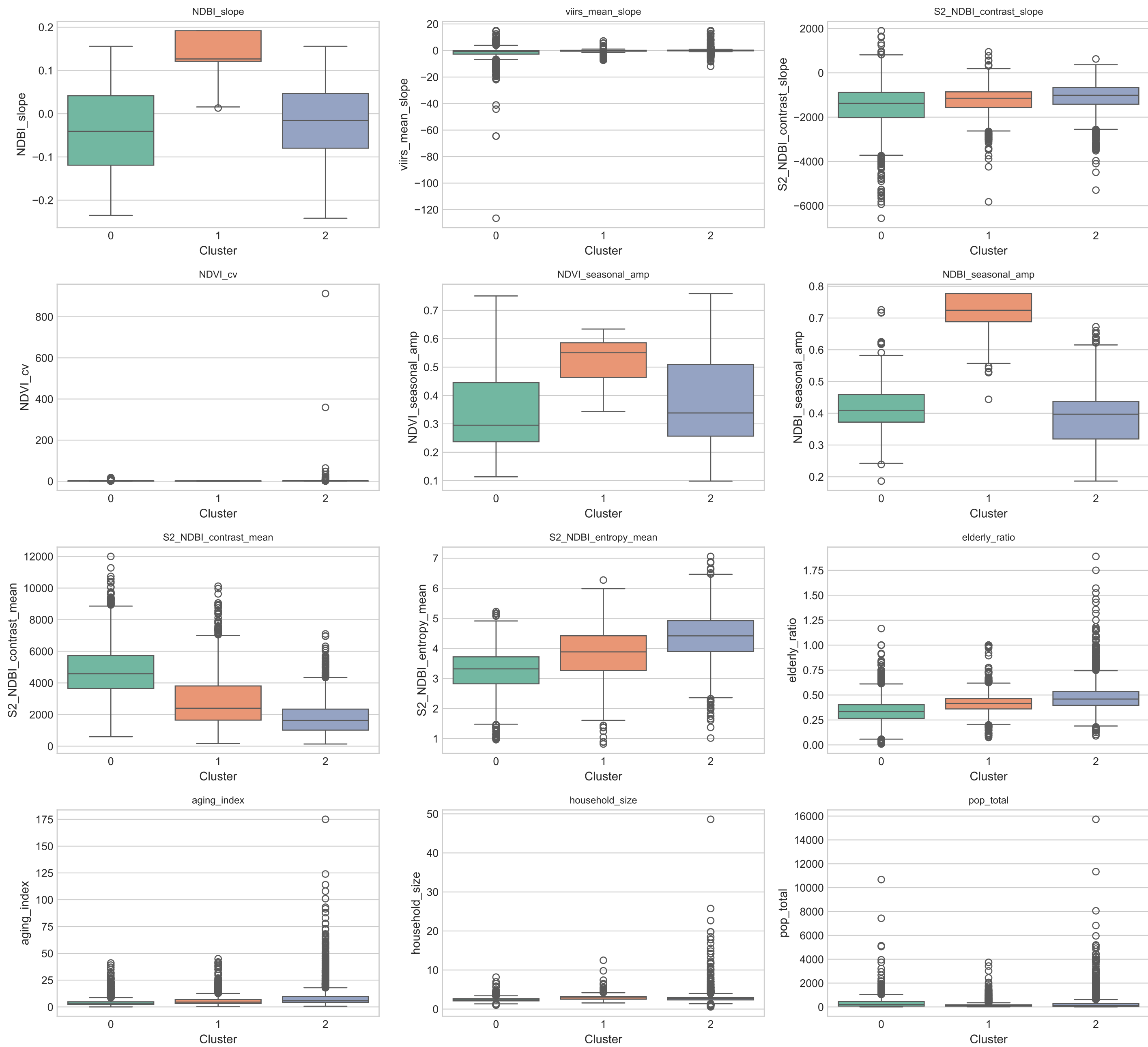
Indicator Distributions by Cluster
