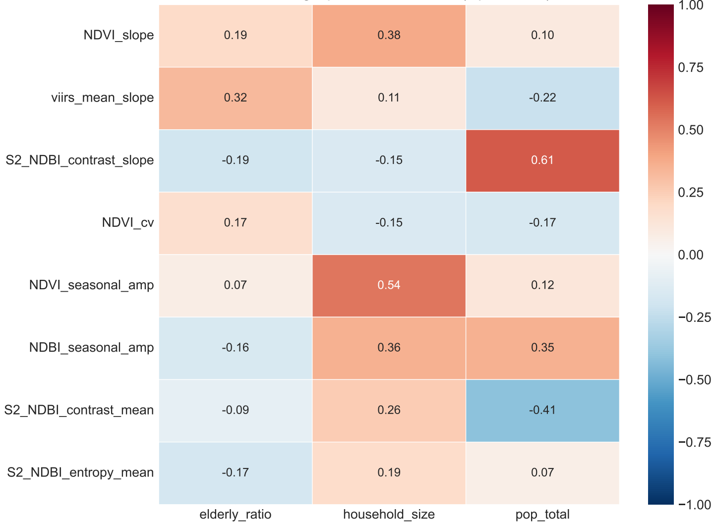
RS-Demographic Correlations (Spearman)
