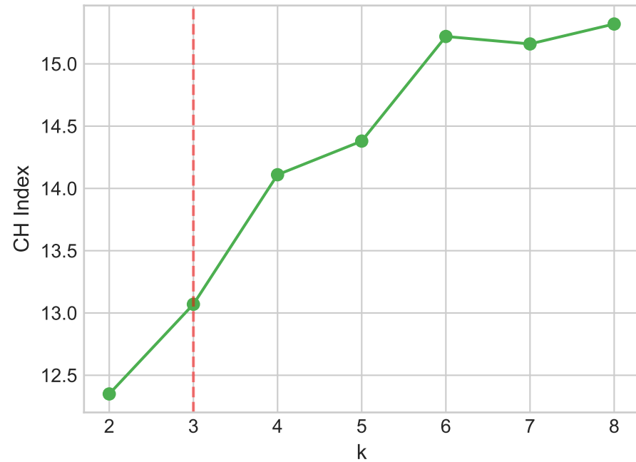
Calinski-Harabasz Index
