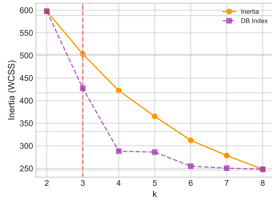
Elbow Method
