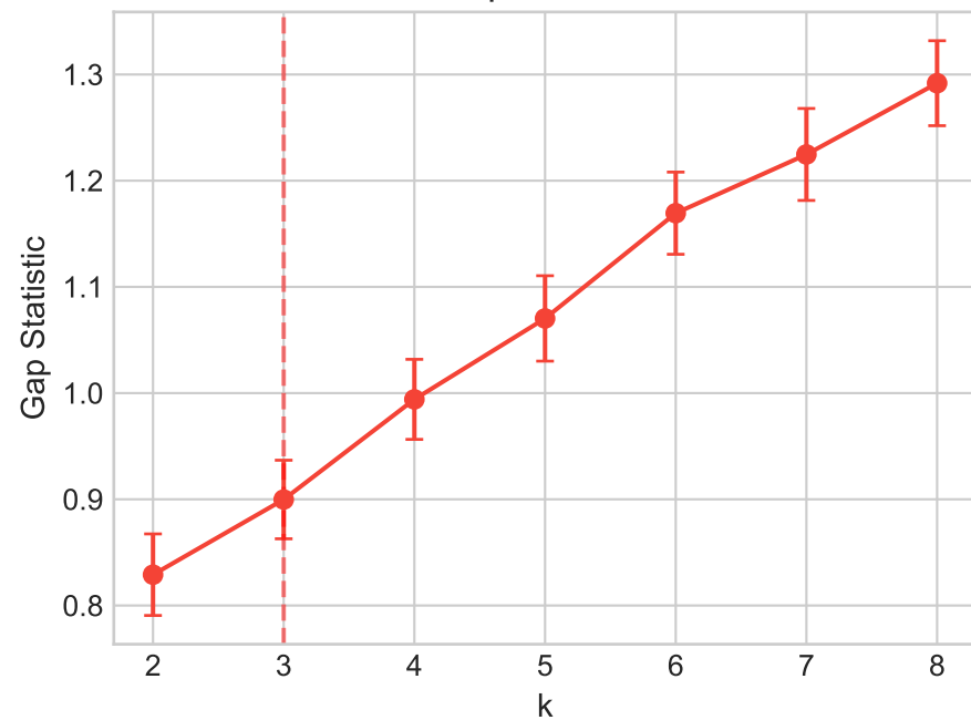
Gap Statistic
