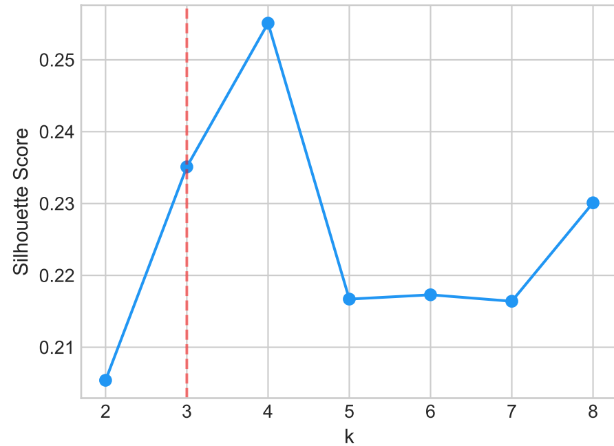
Silhouette Analysis
