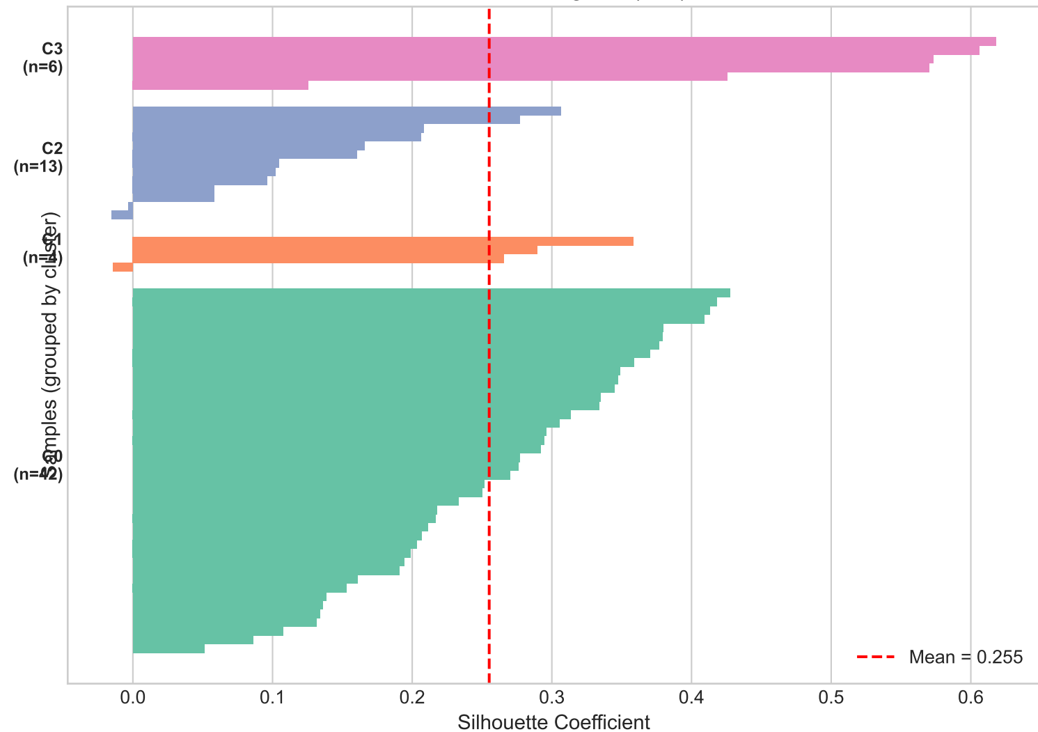
Silhouette Diagram (k=4)
