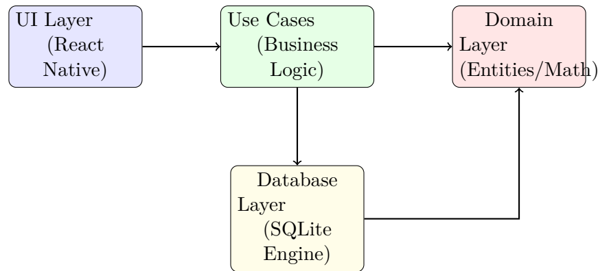
Figure 2: Layer Dependency Diagram in Clean Architecture.
