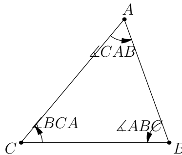
Figure 4: Triangle Sum
