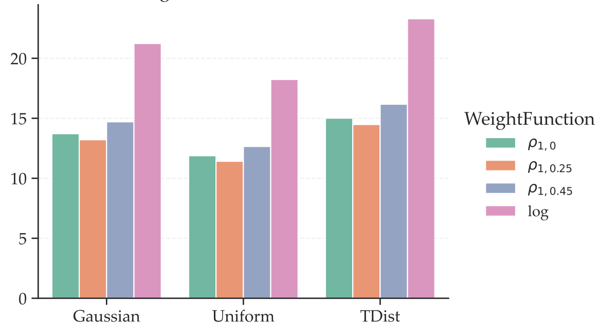
Heterogeneous Variance Inflation
