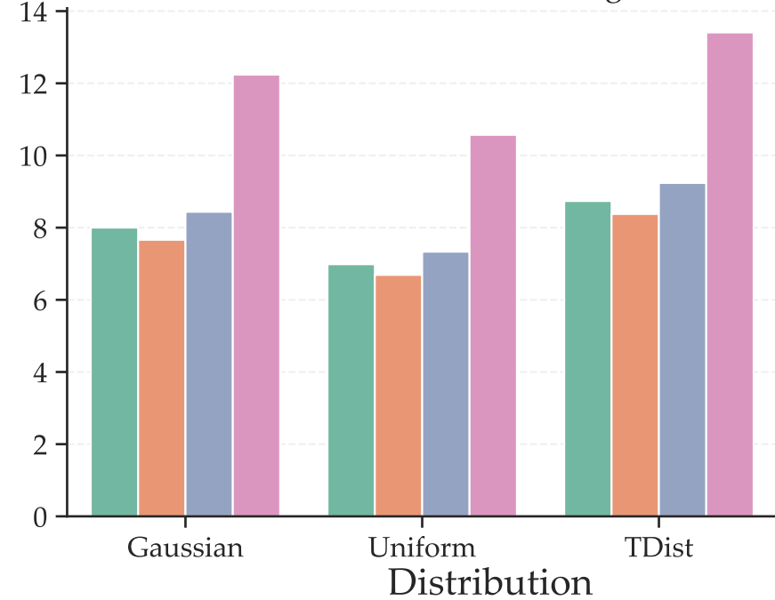
Correlation Structure Change
