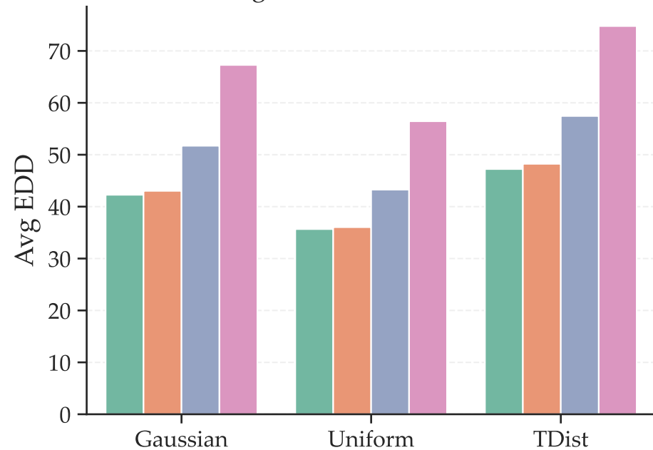
Homogeneous Variance Inflation
