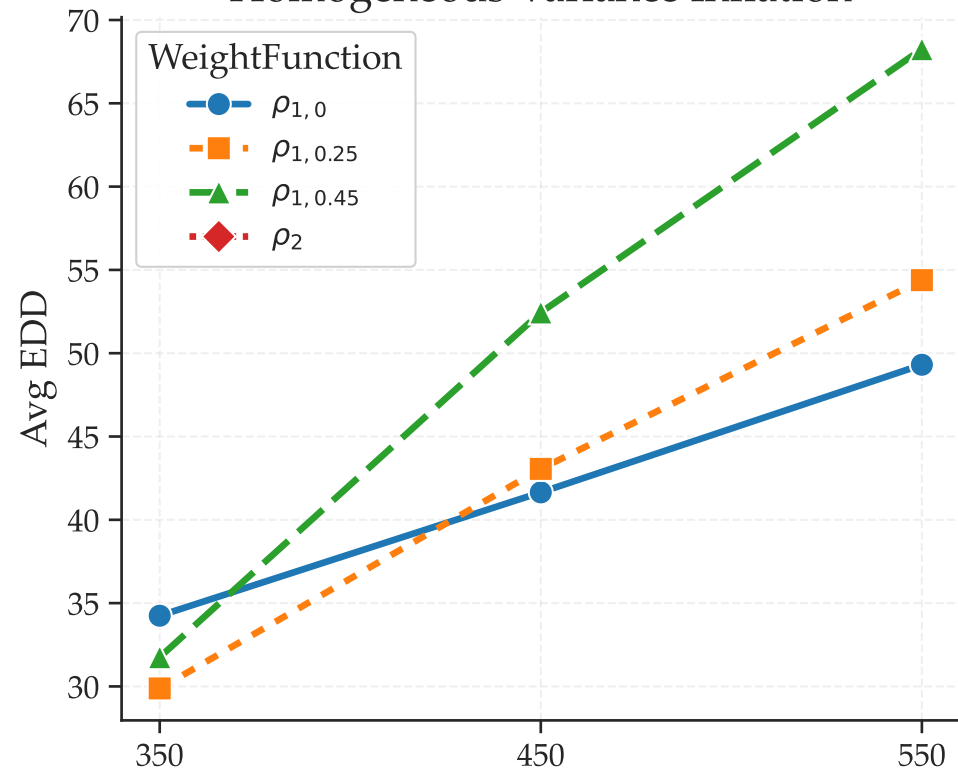
Homogeneous Variance Inflation
