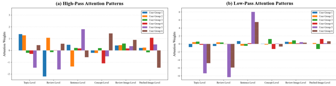
Figure C2. Users’ Attention Divergence Toward Diverse Multi-Granularity Knowledge. Appendix C.4 Qualitative Tracing of Low-Pass and High-Pass Knowledge Selection
