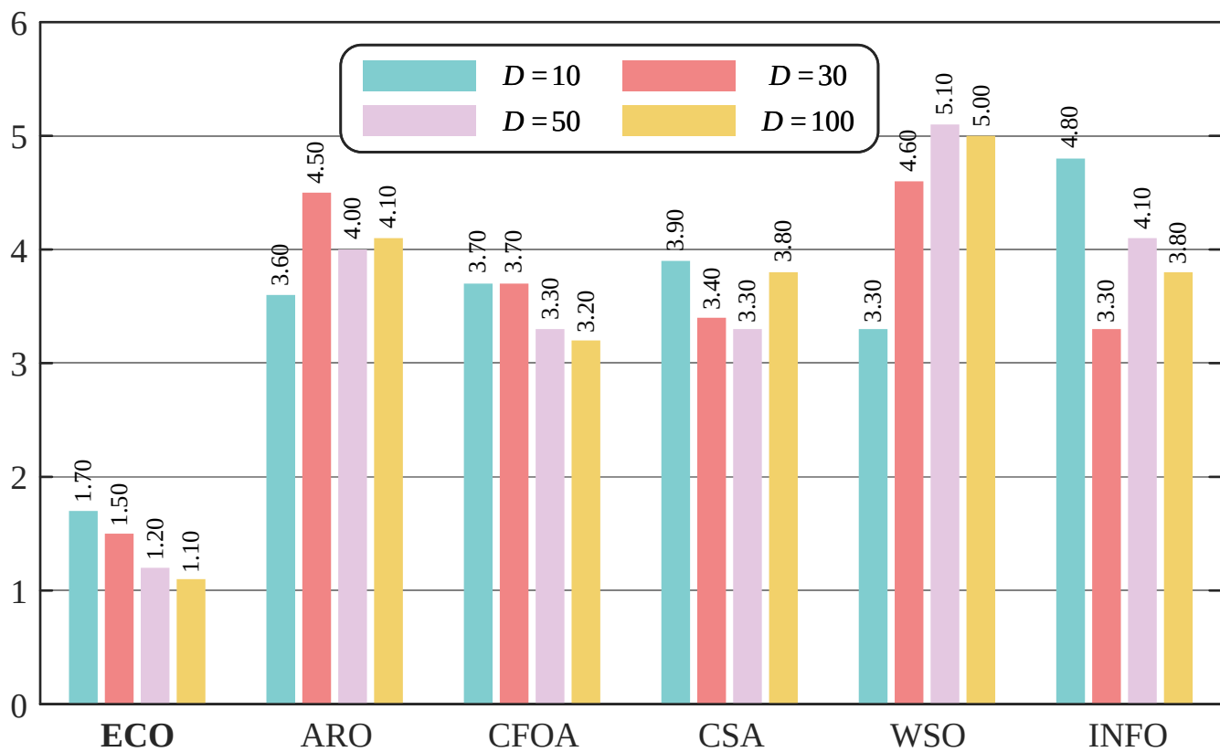
Friedman mean rank
