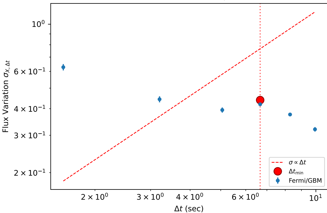
120119A (events=1,065,792) measured \Delta t_{\min} = 6.66 s vs published 0.2 s
