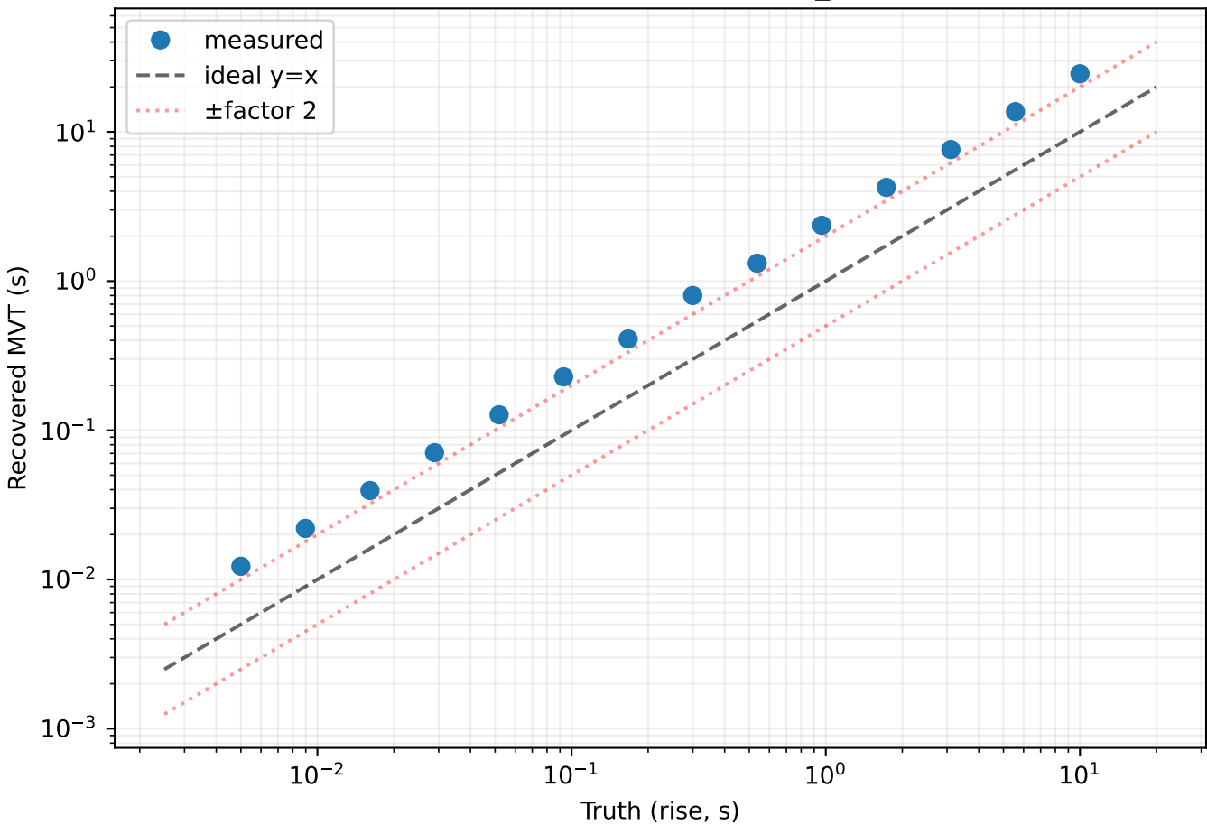
CWT: synthetic recovery (peak_snr=30)
