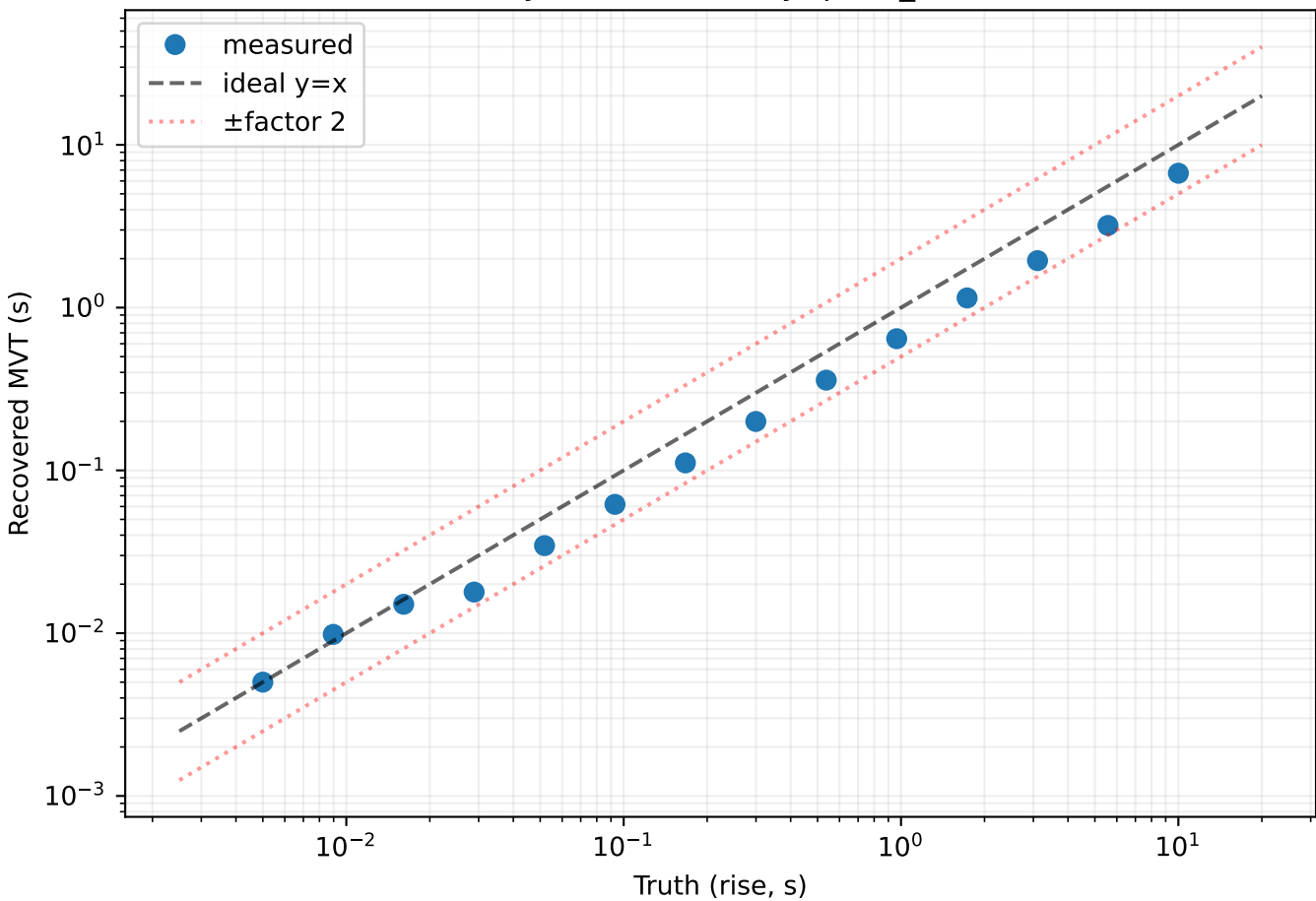
HAAR: synthetic recovery (peak_snr=30)
