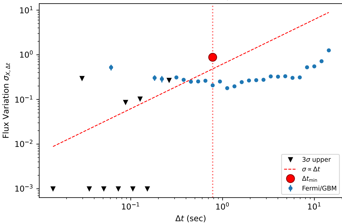
120119A (events=247,594) measured \Delta t_{\min} = 0.78 s vs published 0.2 s
