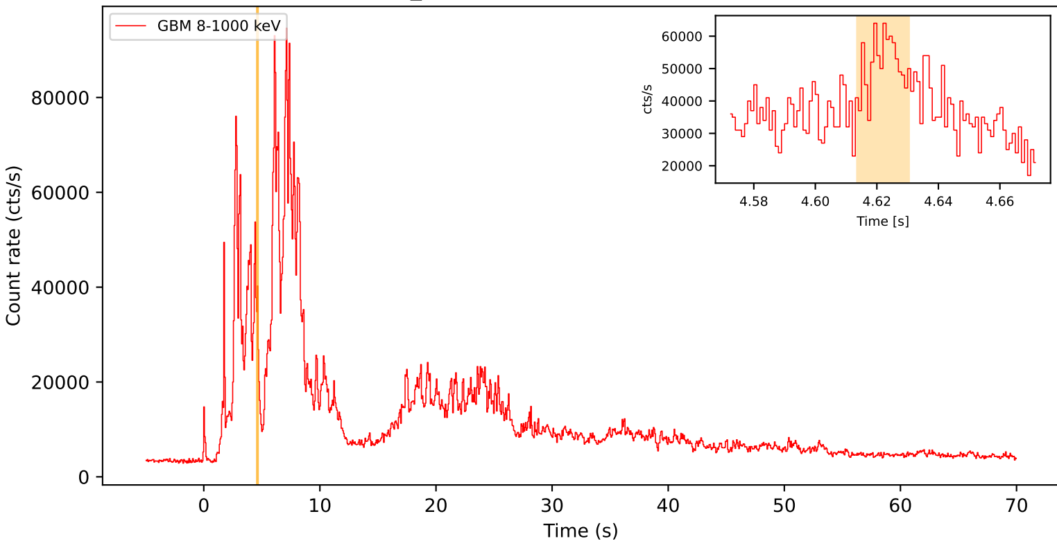
211211A (events=871,254) FWHM_min = 16.86 ms vs published 5.0 ms
