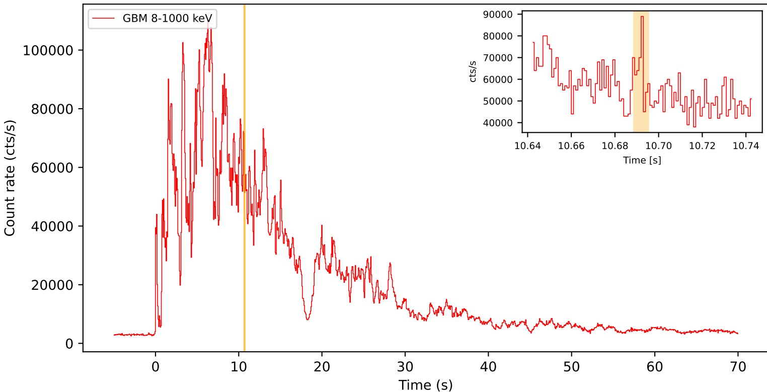
230307A (events=1,487,085) FWHM_min = 6.71 ms vs published 17.0 ms
