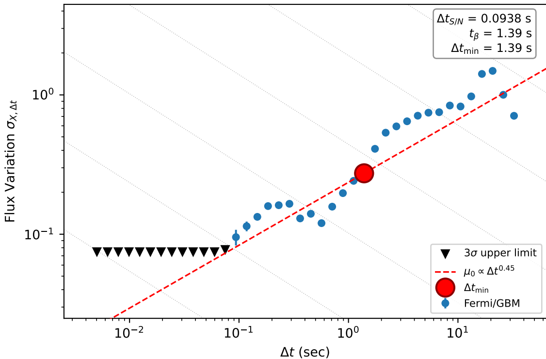
080916A (events=781,703) measured \Delta t_{\min} = 1.39 s vs published 1.09 s
