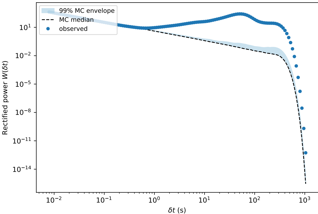
100724B (events=530,126) measured t_{mv} = 0.509 s vs published 0.3 s
