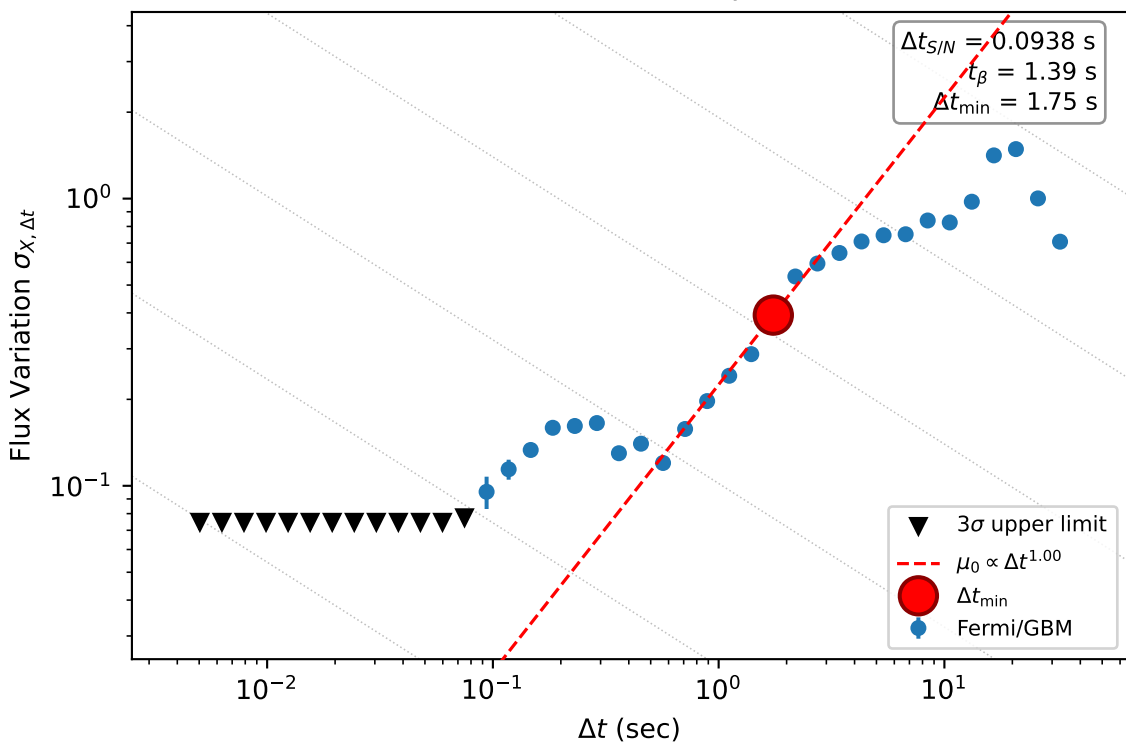
080916A (events=781,703) measured \Delta t_{\min} = 1.75 s vs published 1.09 s
