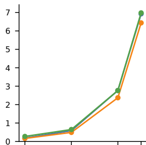
GSEA (1,000 perm.)
