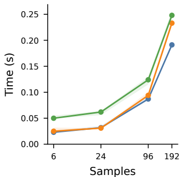
FRY (50 sets)
