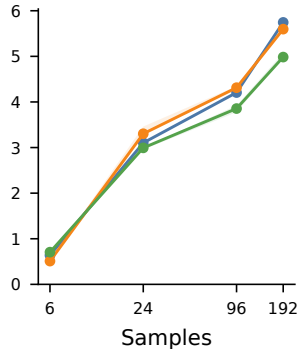
GSEA (1,000 perm.)
