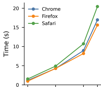
FRY (50 sets)
