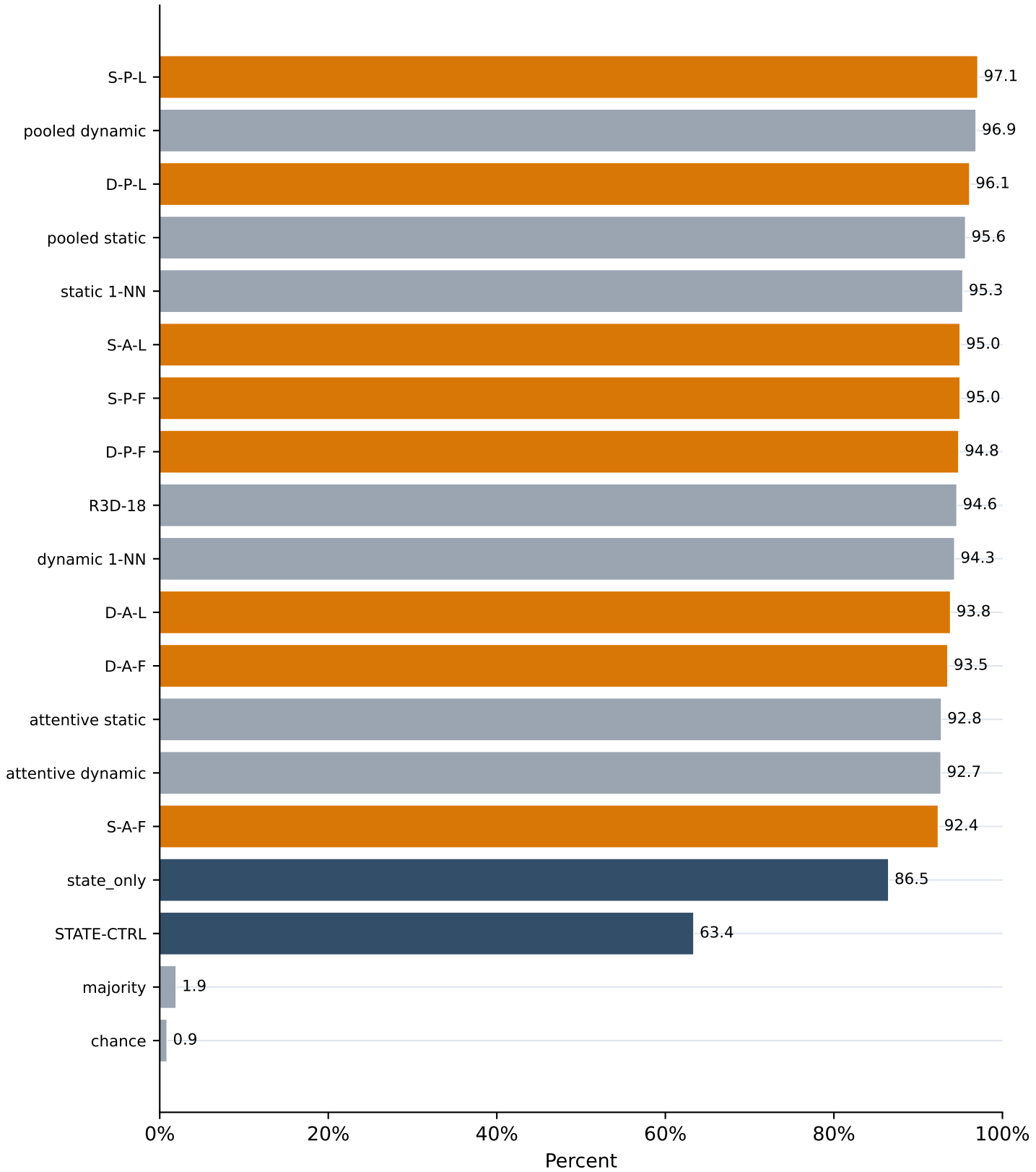
Top-1 accuracy
