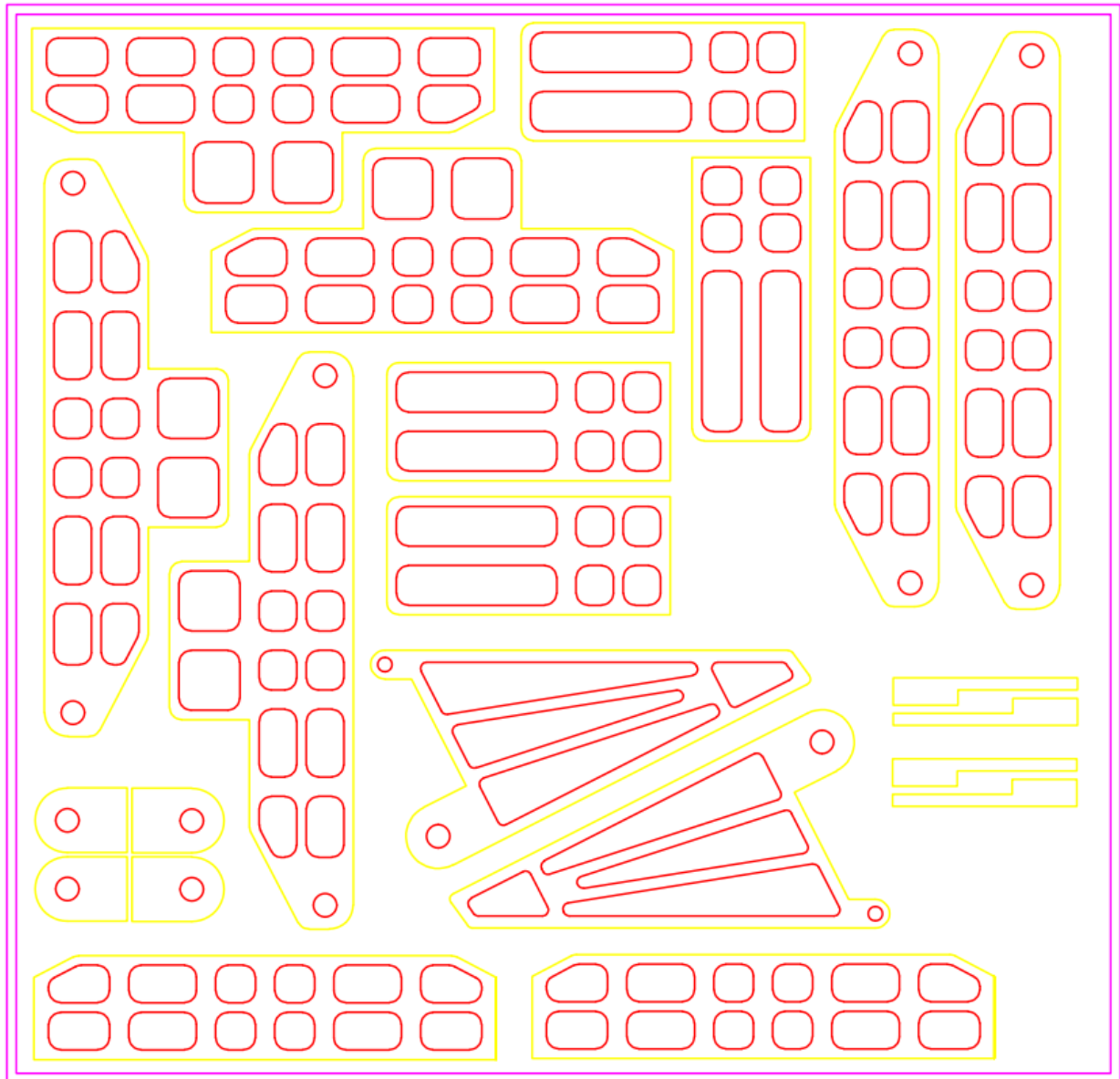
Figure 1: Image of the first AutoCAD drawing with dimensions 930 x 900.
