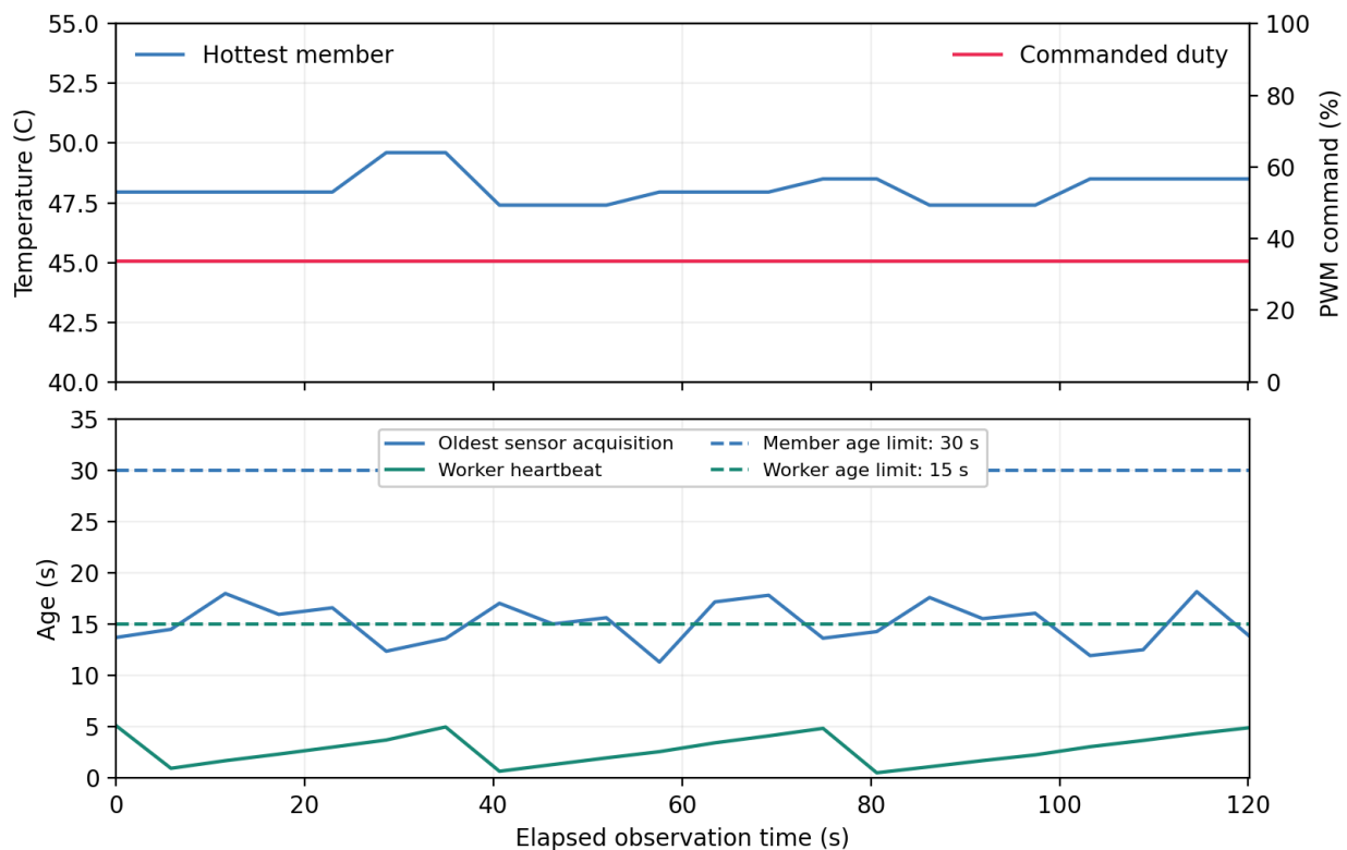
Stable v1 runtime: actual sensor clocks PWM command is not measured RPM
