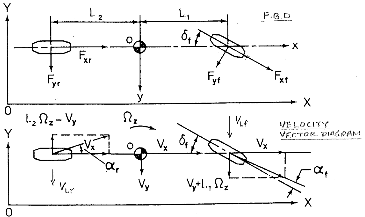
Fig. 5.17 Simplified vehicle model for analysis of transient motions.
