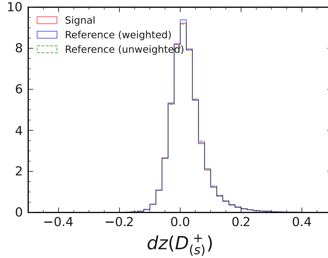
Normalized Distributions for D^+ \rightarrow \eta_{\gamma\gamma} K^+ and D^+ \rightarrow \eta_{\gamma\gamma} \pi^+
