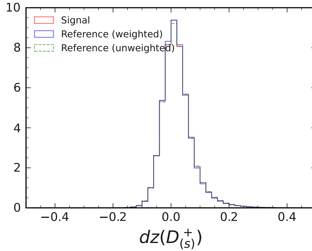
Normalized Distributions for D^+ \rightarrow \eta_{3\pi} K^+ and D^+ \rightarrow \eta_{3\pi} \pi^+
