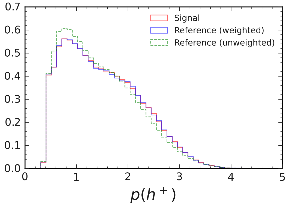
Normalized Distributions for D_s^+ \rightarrow \eta_{\gamma\gamma} \pi^+ and D^+ \rightarrow K_S^0 \pi^+ in \cos \theta^* < 0
