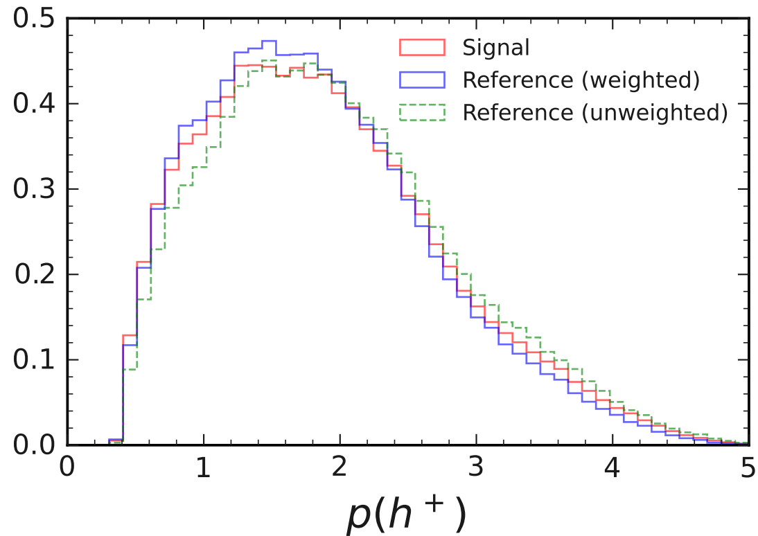
Normalized Distributions for D_s^+ \rightarrow \eta_{\gamma\gamma} K^+ and D_s^+ \rightarrow K_S^0 K^+ in \cos \theta^* > 0
