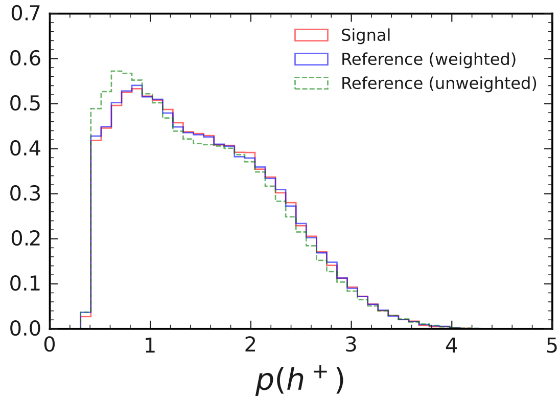
Normalized Distributions for D_s^+ \rightarrow \eta_{3\pi} \pi^+ and D^+ \rightarrow K_S^0 \pi^+ in \cos \theta^* < 0
