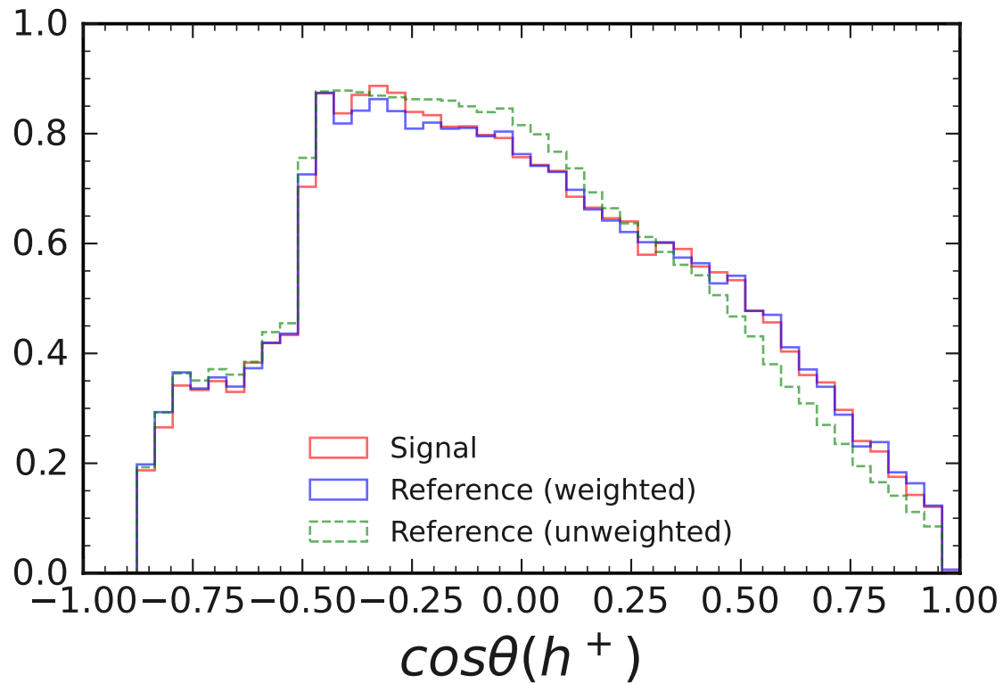
Normalized Distributions for D_s^+ \rightarrow \eta_{3\pi} \pi^+ and D^+ \rightarrow K_S^0 \pi^+ in \cos \theta^* < 0
