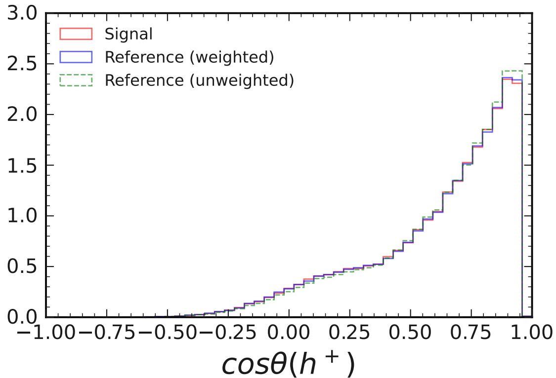
Normalized Distributions for D_s^+ \rightarrow \eta_{3\pi} K^+ and D_s^+ \rightarrow K_S^0 K^+ in \cos \theta^* > 0
