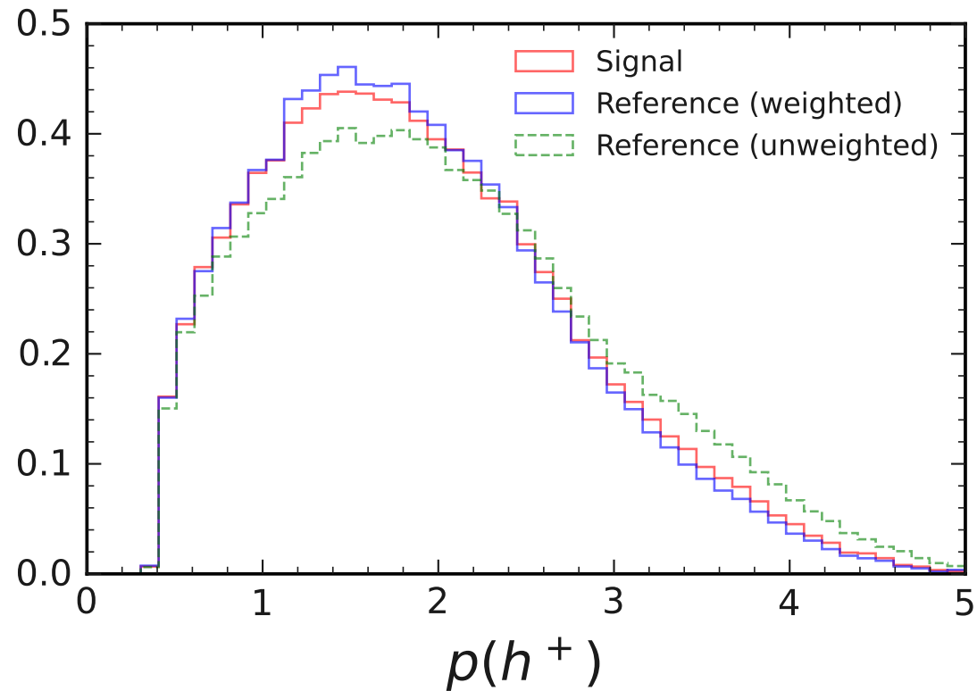
Normalized Distributions for D_s^+ \rightarrow \eta_{3\pi} K^+ and D_s^+ \rightarrow K_S^0 K^+ in \cos \theta^* > 0
