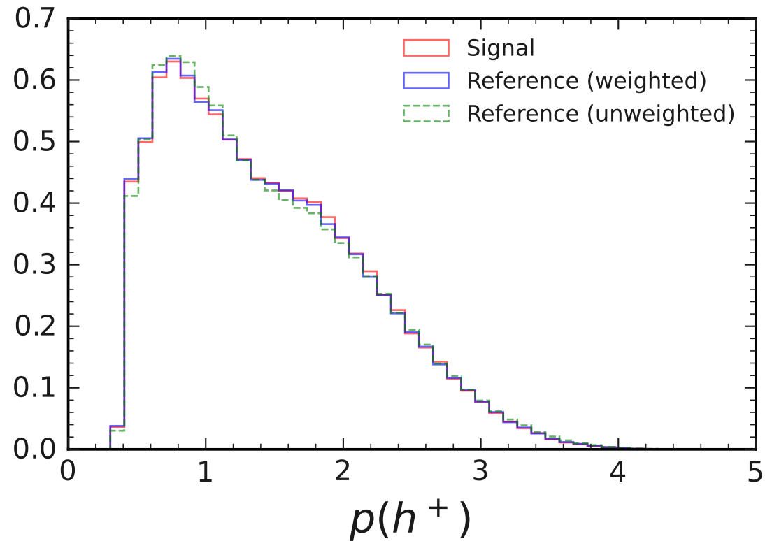
Normalized Distributions for D^+ \rightarrow \eta_{\gamma\gamma} \pi^+ and D^+ \rightarrow K_S^0 \pi^+ in \cos \theta^* < 0
