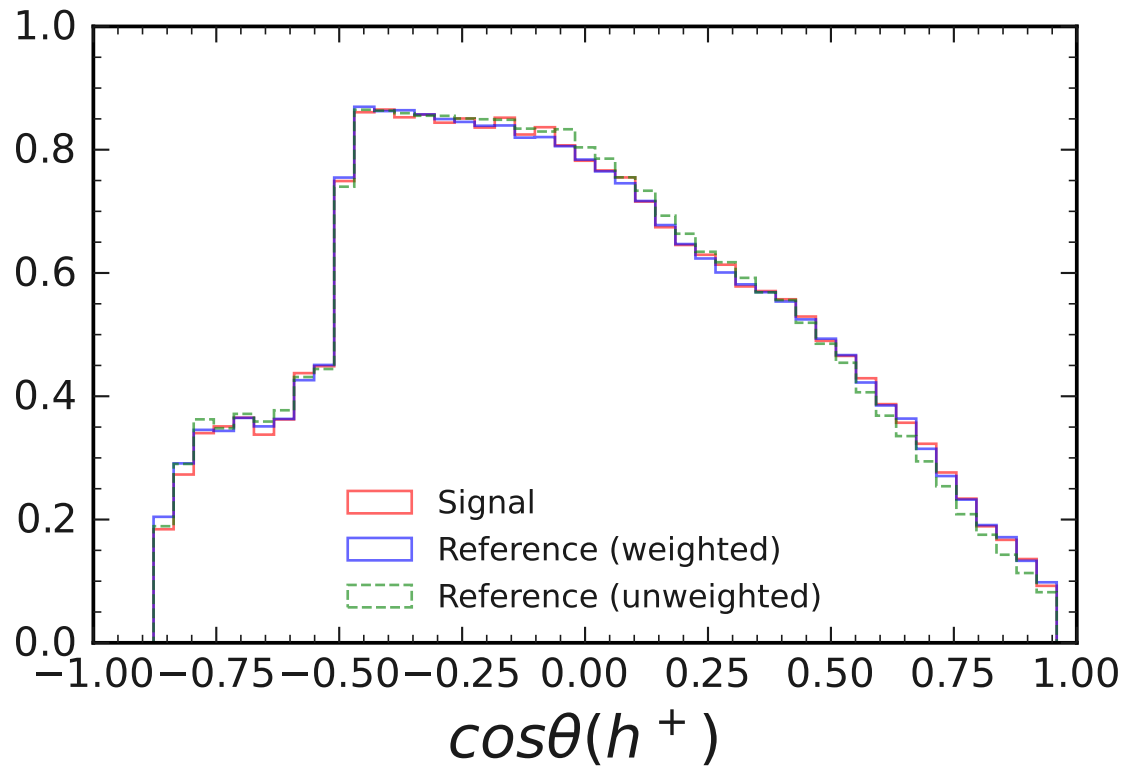
Normalized Distributions for D^+ \rightarrow \eta_{\gamma\gamma} \pi^+ and D^+ \rightarrow K_S^0 \pi^+ in \cos \theta^* < 0
