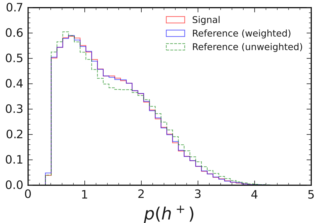
Normalized Distributions for D^+ \rightarrow \eta_{3\pi} \pi^+ and D^+ \rightarrow K_S^0 \pi^+ in \cos \theta^* < 0
