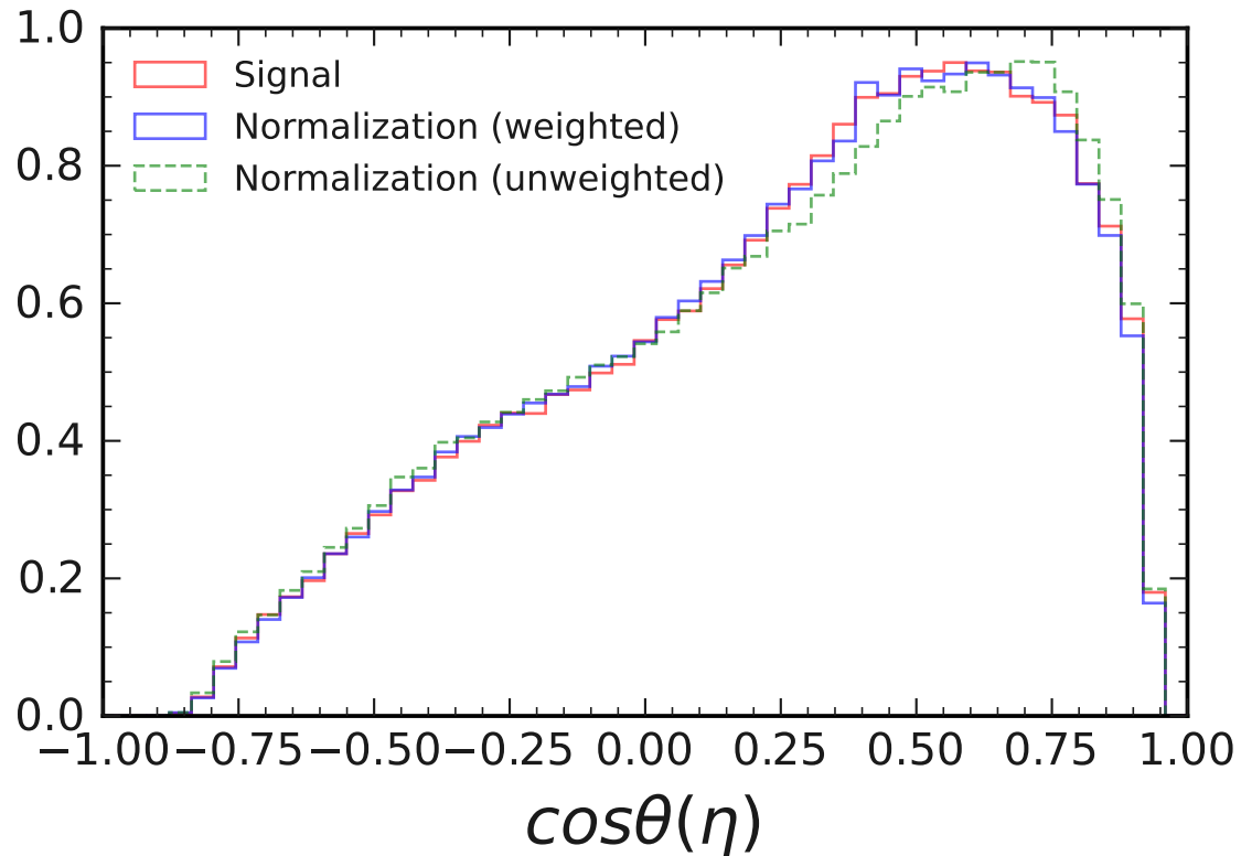
Distributions for D_s^+ \rightarrow \eta_{3\pi} K^+ and D_s^+ \rightarrow \eta_{3\pi} \pi^+
