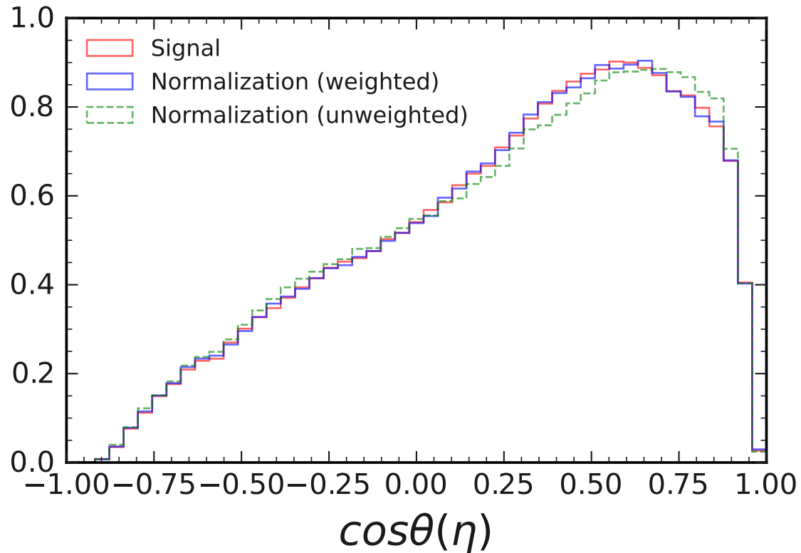
Distributions for D^+ \rightarrow \eta_{\gamma\gamma} K^+ and D^+ \rightarrow \eta_{\gamma\gamma} \pi^+
